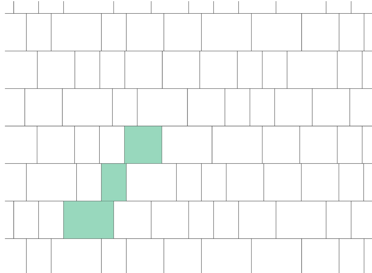
I PAVER PATTERN - Random Running Bond
