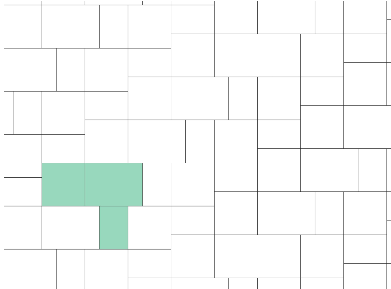
H PAVER PATTERN - Herringbone
