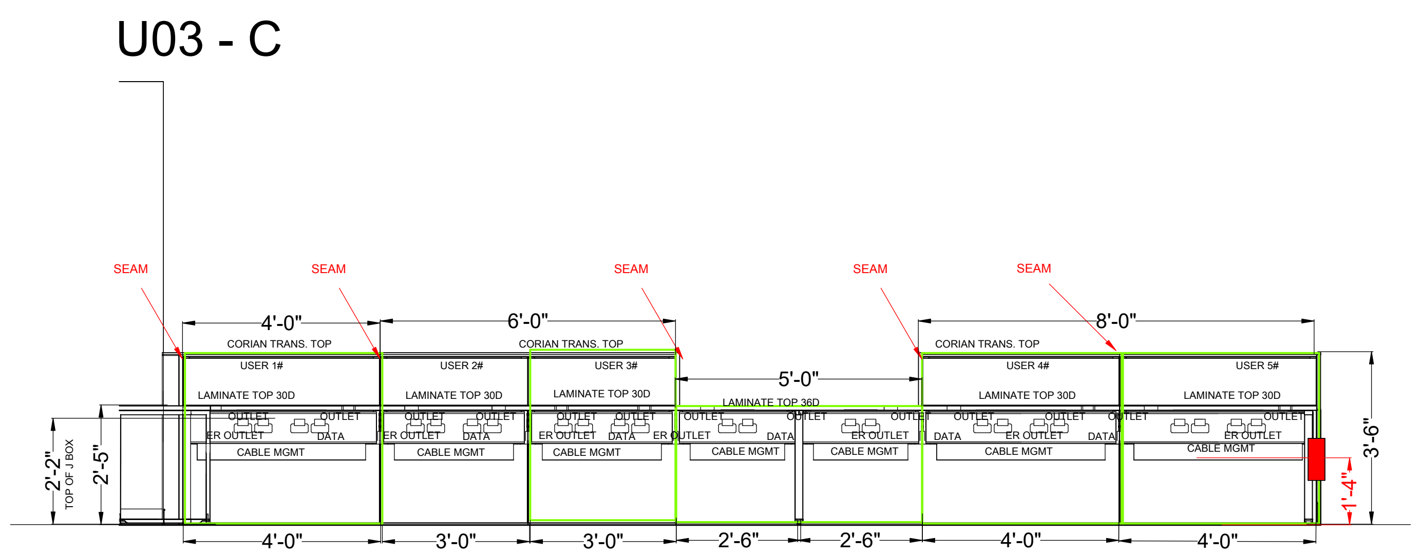
U3 NURSE STATION ELEVATION VIEW SCALE: 1/2"=1"
