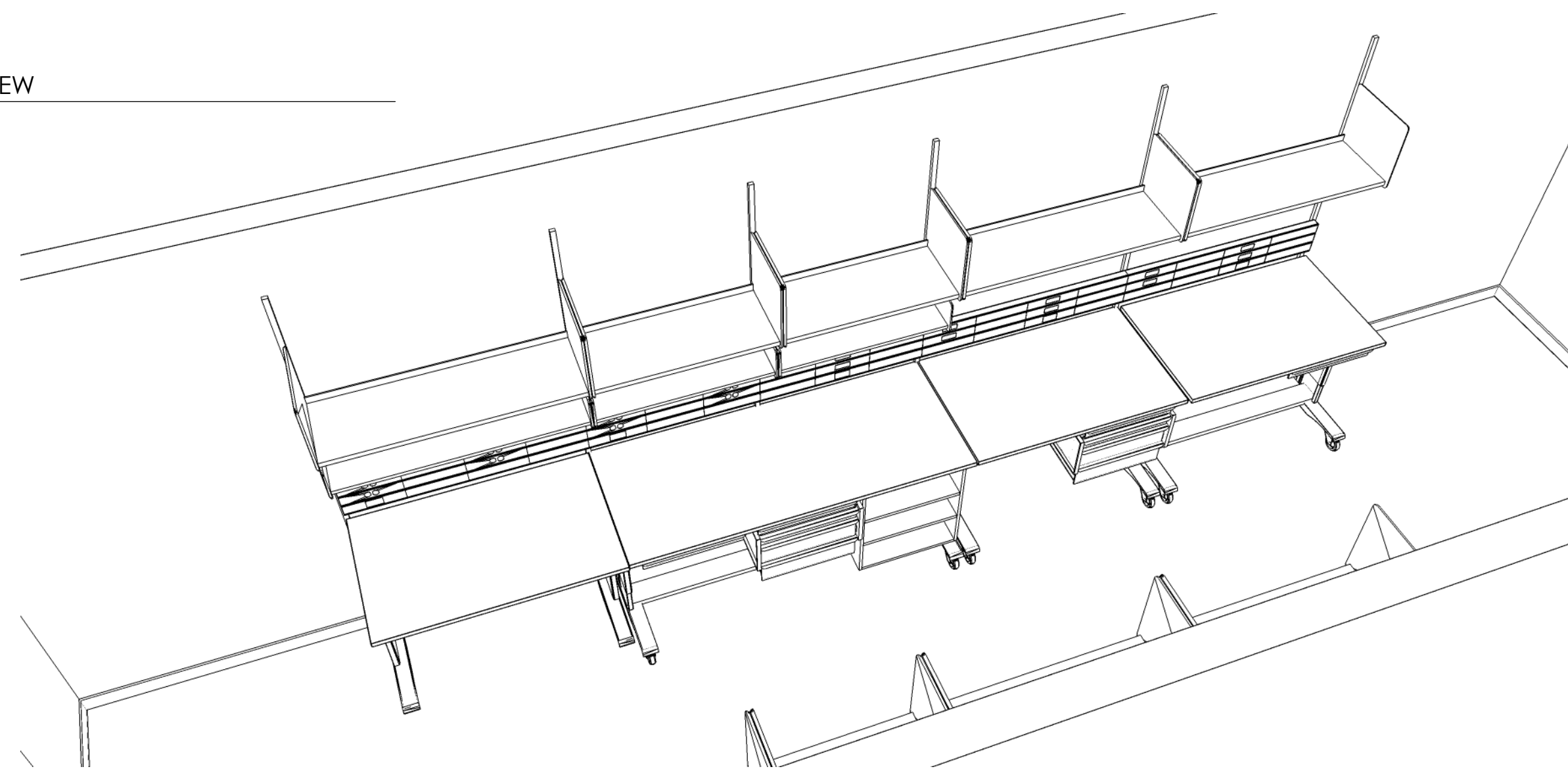
D LAB ISOMETRIC VIEW SCALE: NTS
