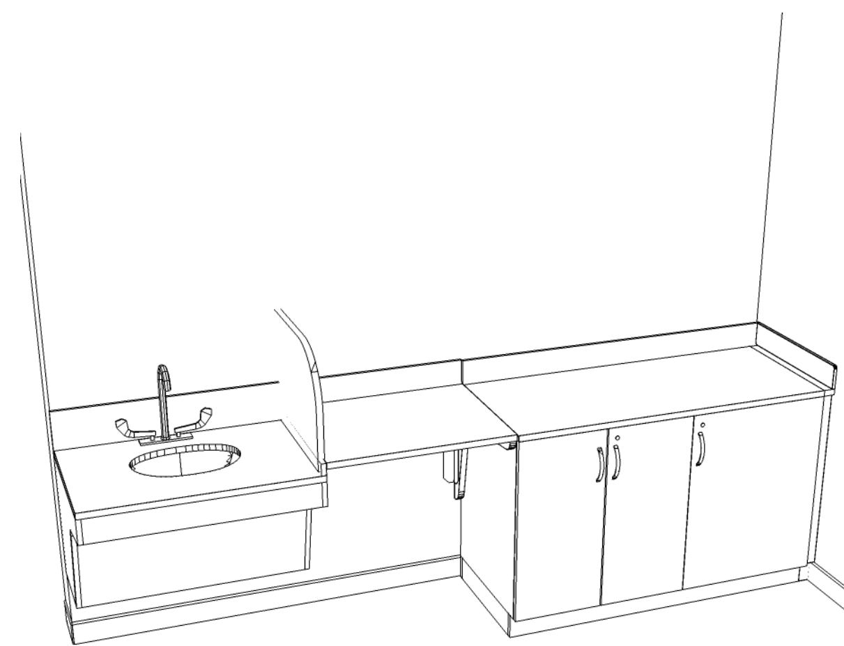
E7B RESUS 11 ISOMETRIC VIEW SCALE: NTS
