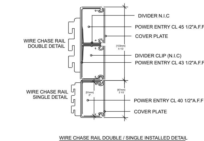
WIRE CHASE 3 TO 1 SCALE 3" = 1'-0"
