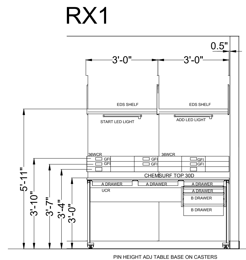
RX PHARMACY ELEVATION VIEW SCALE: 1/2"=1"
