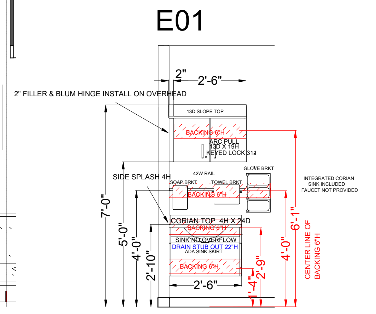
1 EXAM TYPICAL SINK LEFT ELEVATION VIEW SCALE: 1/2"=1"
