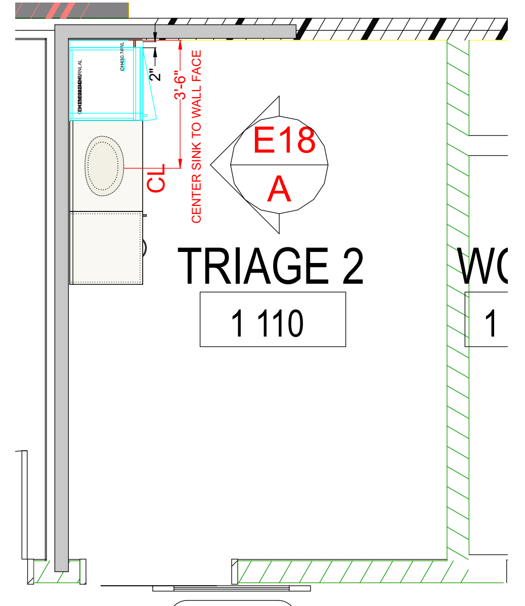
18 TRIAGE 2 PLAN VIEW SCALE: 3/8"=1"
