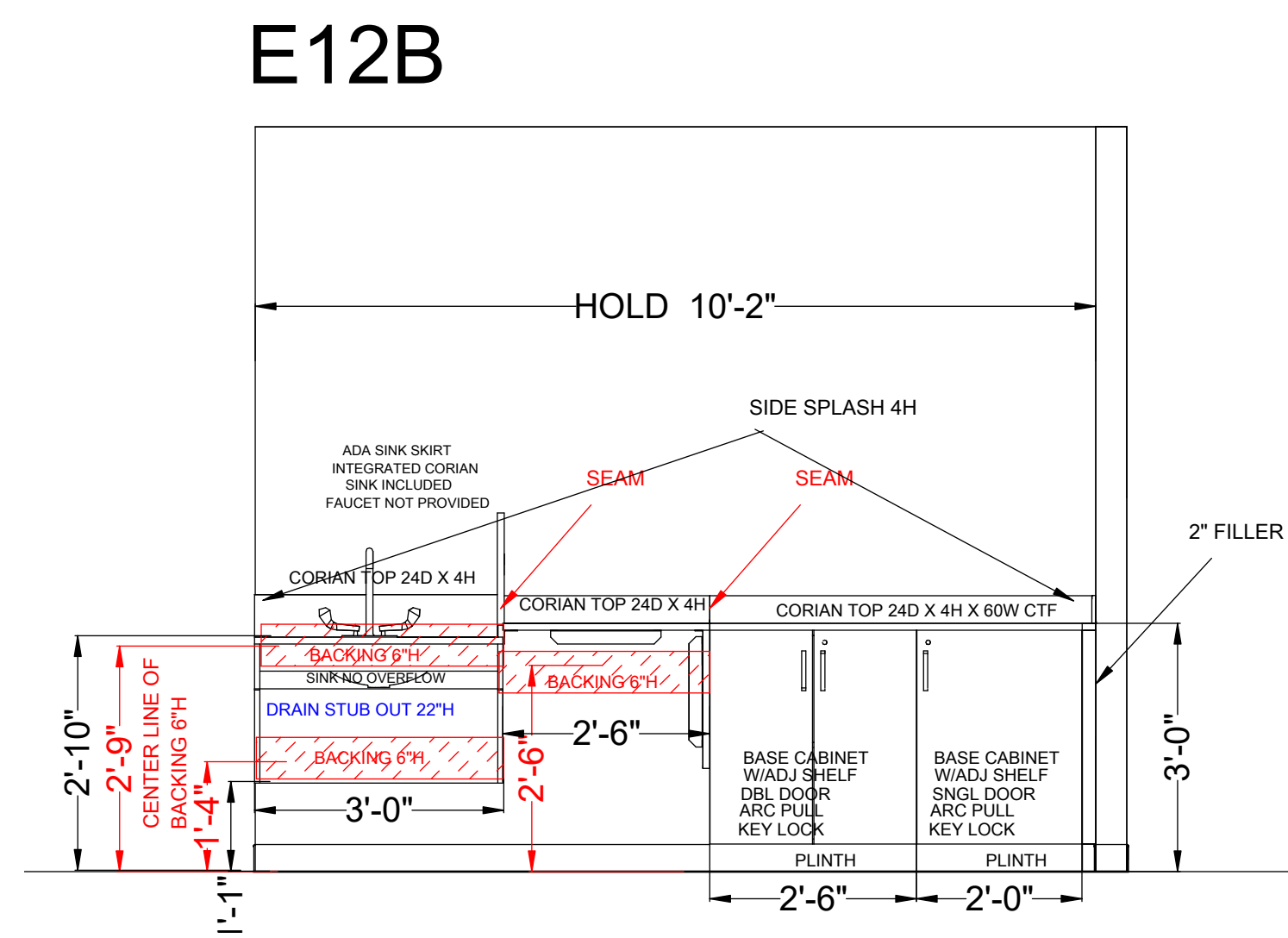
E12B MEDS ELEVATION VIEW SCALE: 1/2"=1"
