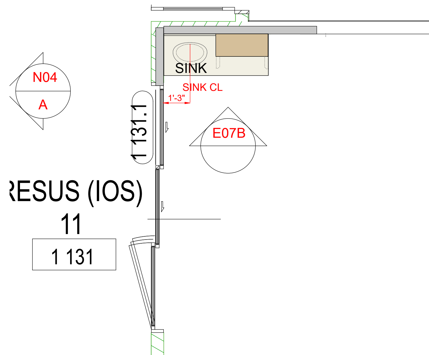
E7B RESUS 11 PLAN VIEW SCALE: 3/8"=1"
