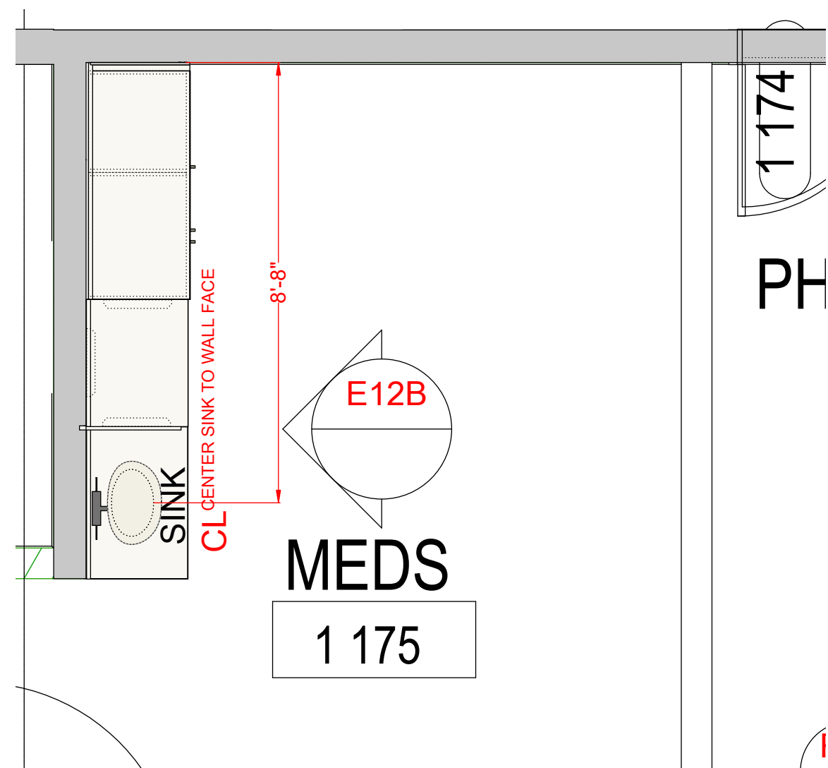
E12B MEDS PLAN VIEW SCALE: 3/8"=1"
