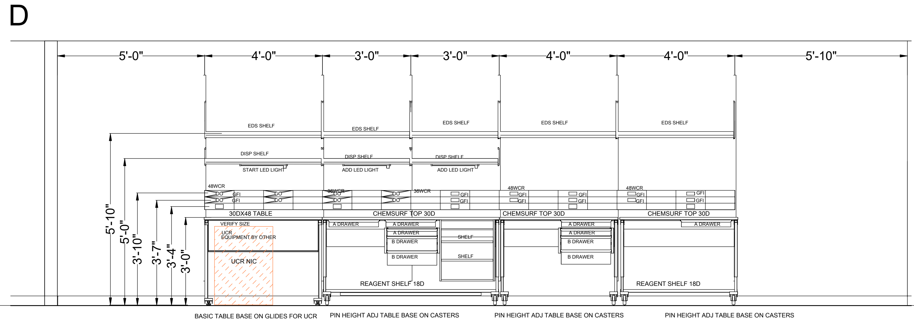
D LAB ELEVATION VIEW SCALE: 1/2"=1"
