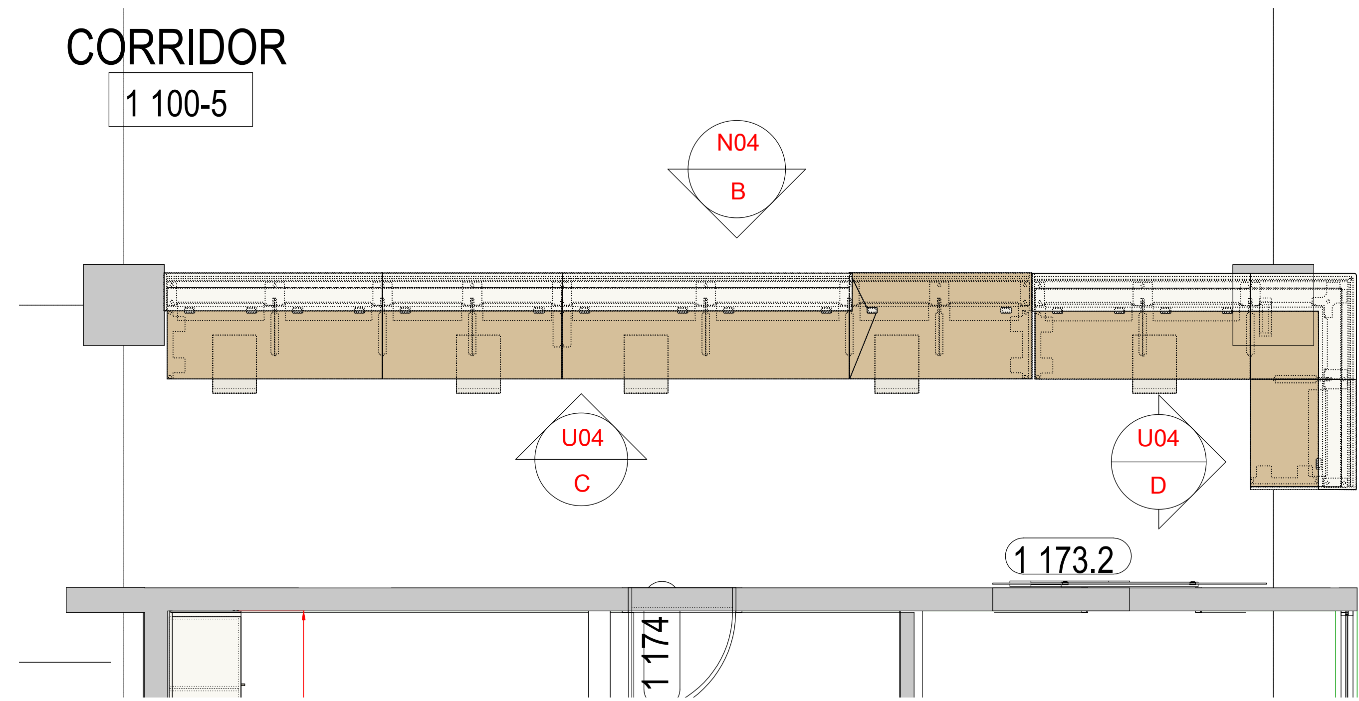
N4 NURSE STATION PLAN VIEW SCALE: 3/8"=1"
