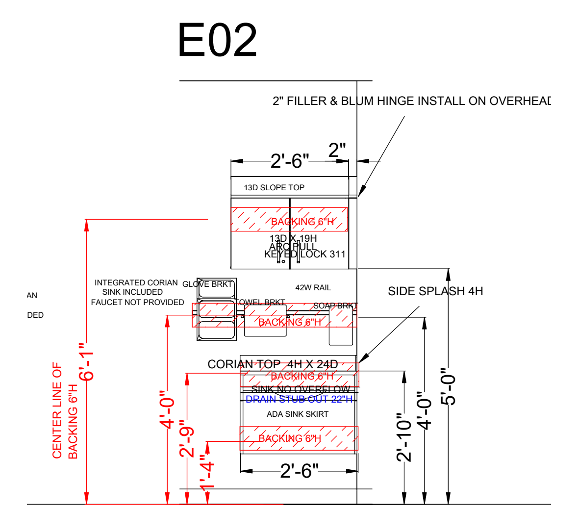
2 EXAM TYPICAL SINK RIGHT ELEVATION VIEW SCALE: 1/2"=1"
