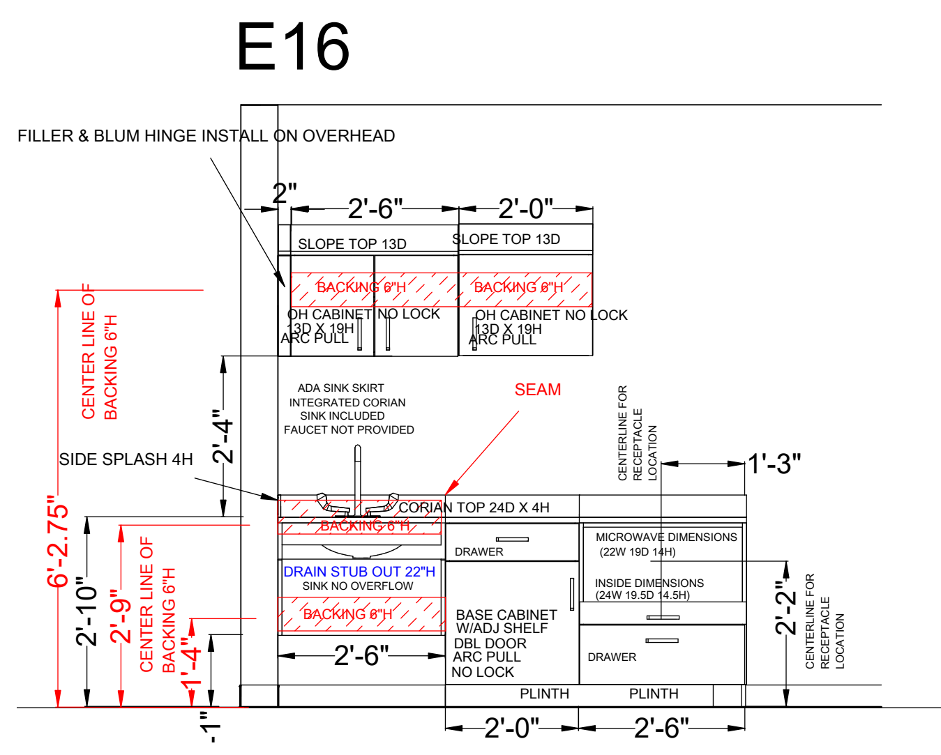
16 EMS ELEVATION VIEW SCALE: 1/2"=1"
