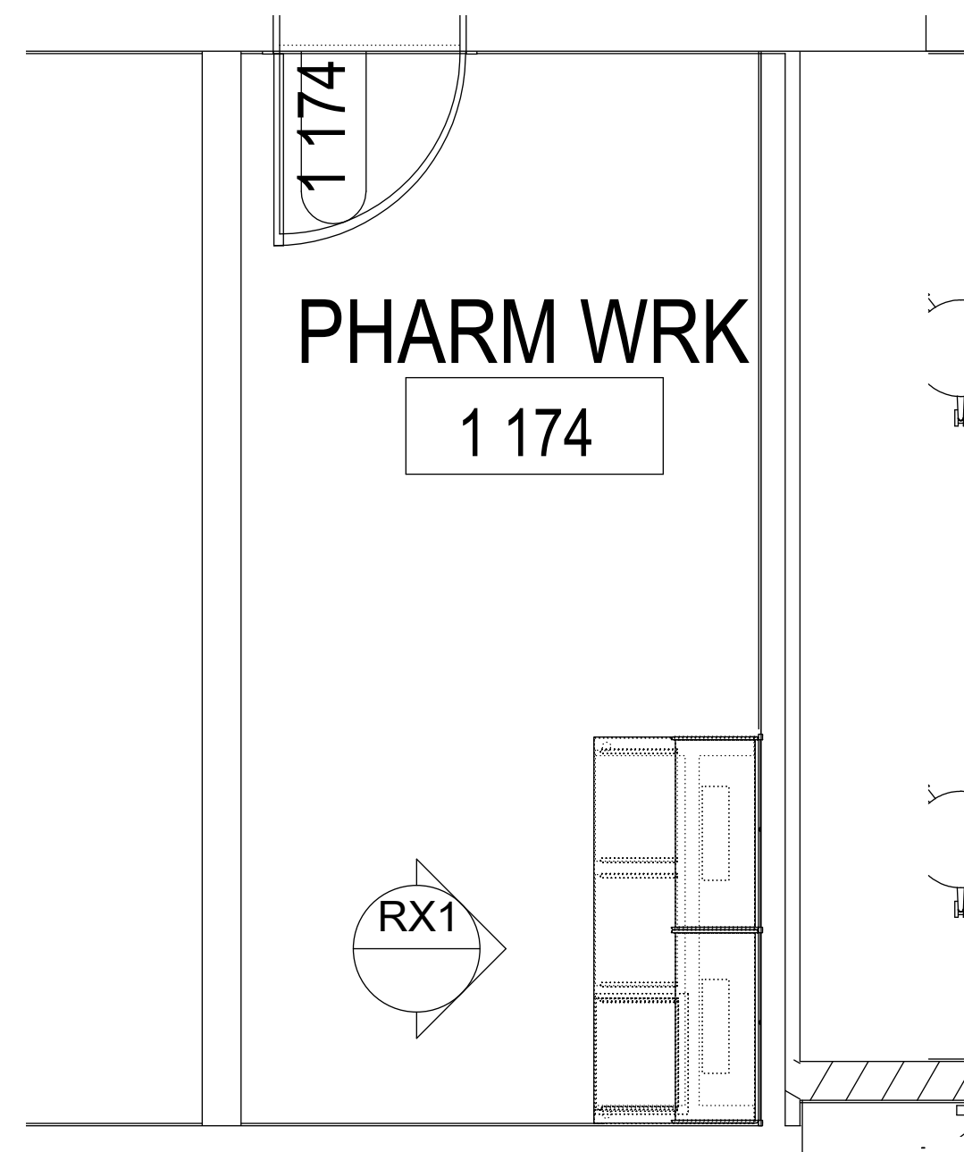
RX PHARMACY PLAN VIEW SCALE: 3/8"=1"
