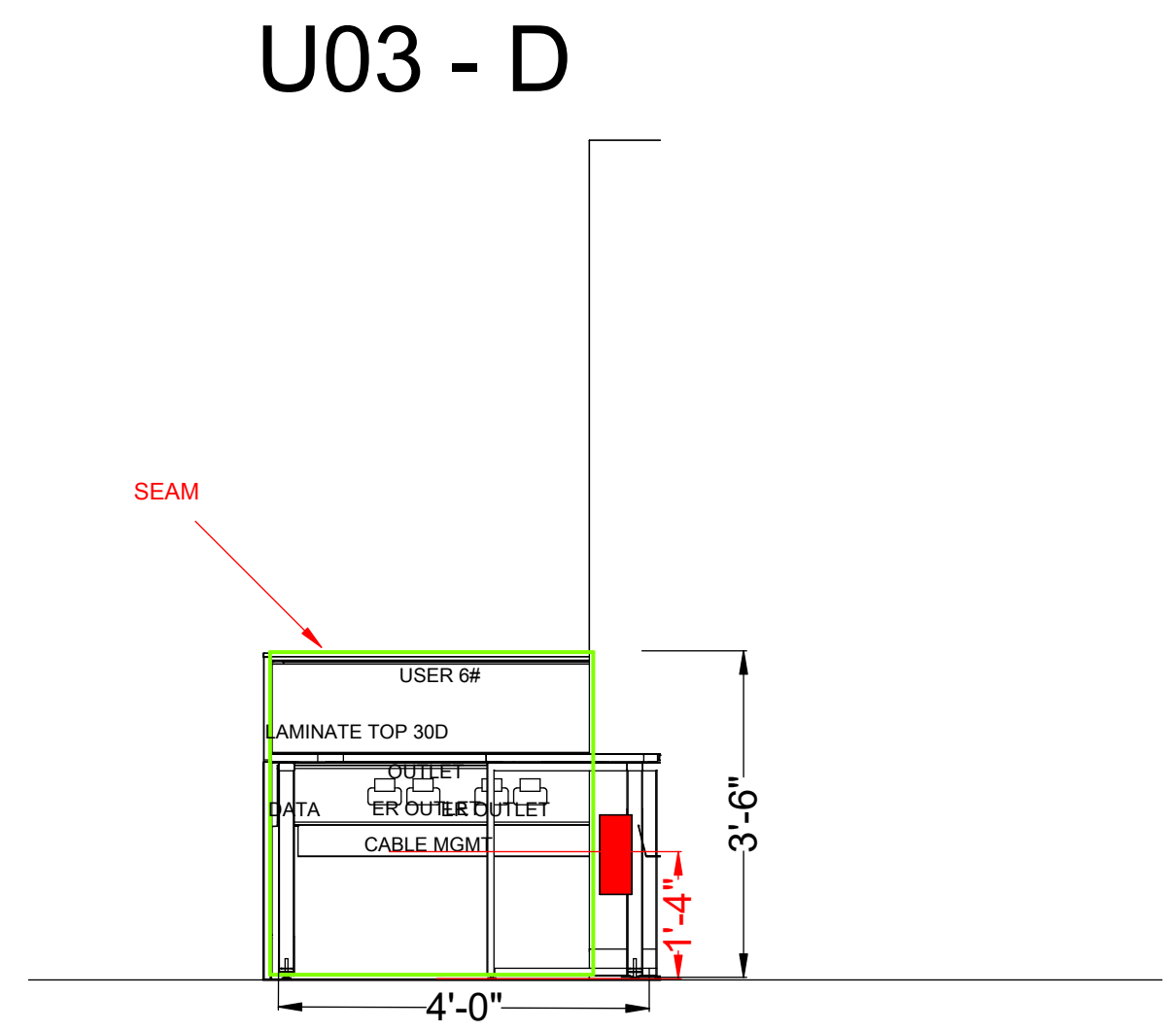
U3 NURSE STATION ELEVATION VIEW SCALE: 1/2"=1"
