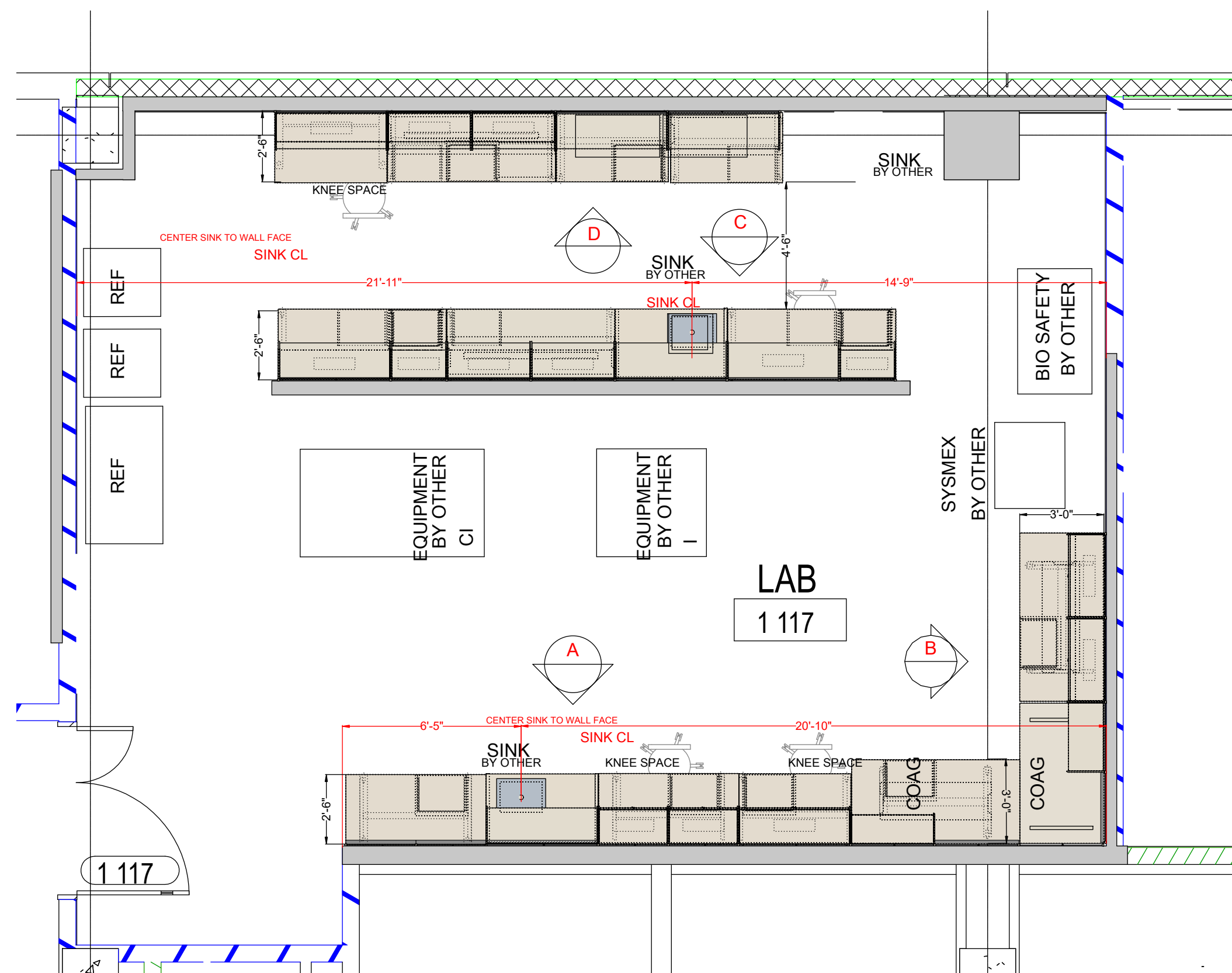
A LAB 1041 PLAN VIEW SCALE: 3/8"=1'
