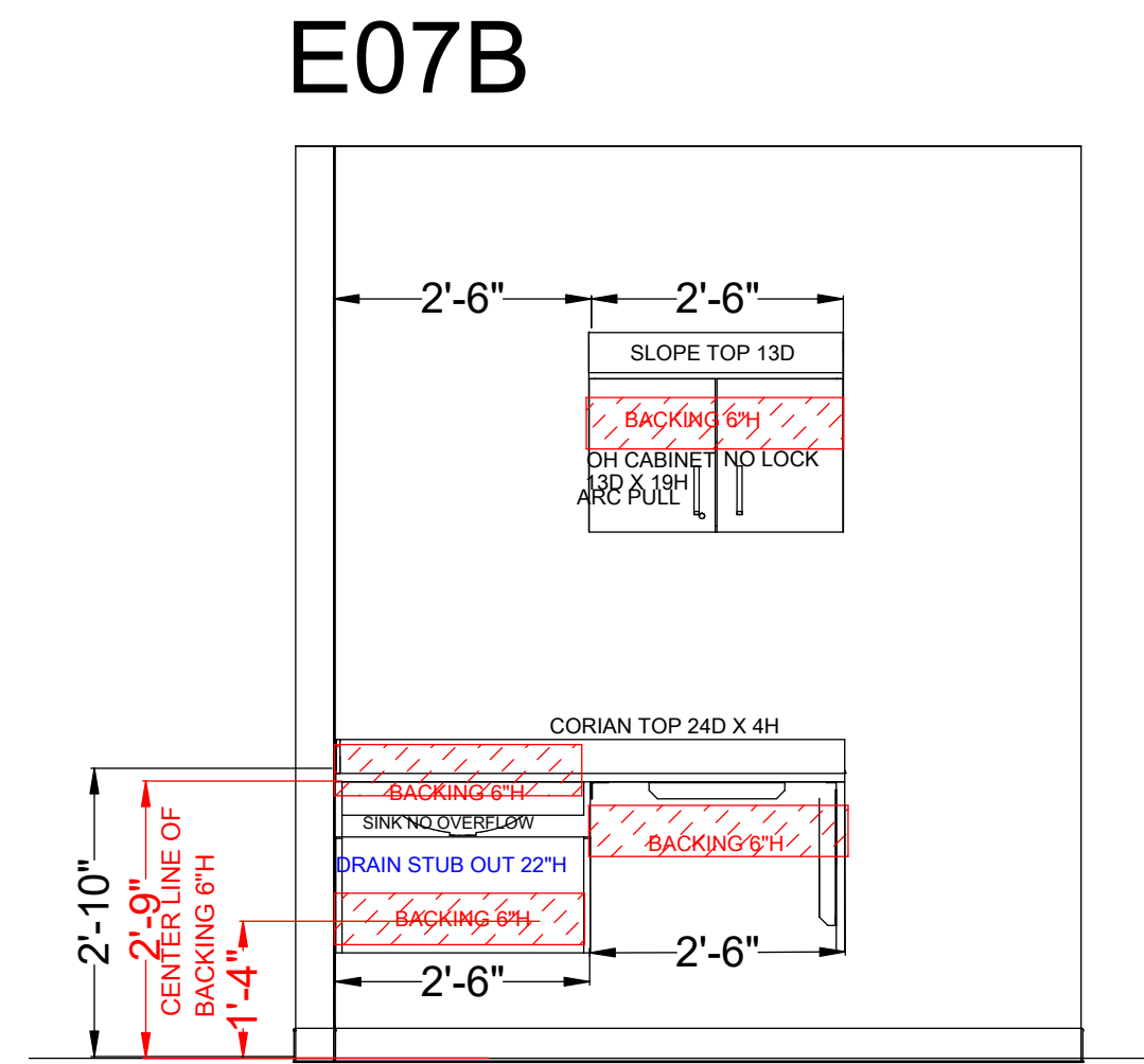
E7B RESUS 11 ELEVATION VIEW SCALE: 1/2"=1"
