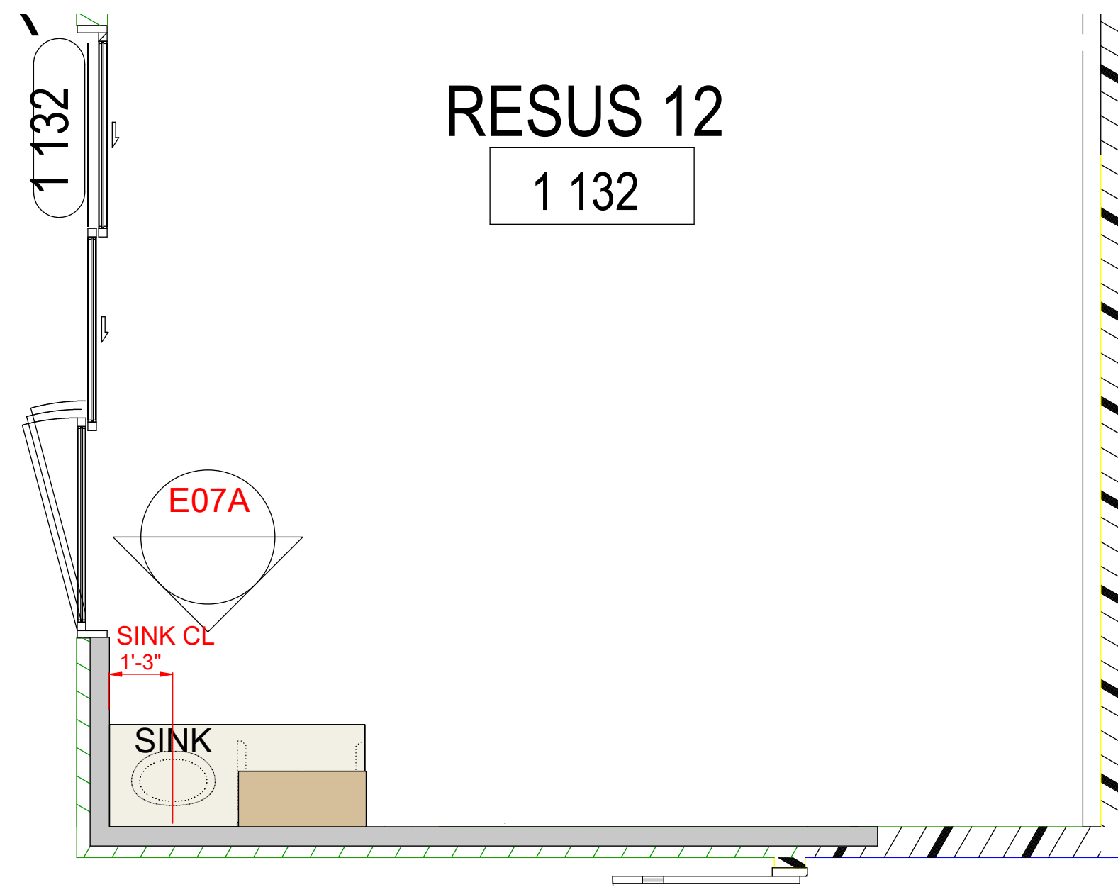
E7A RESUS 12 PLAN VIEW SCALE: 3/8"=1"
