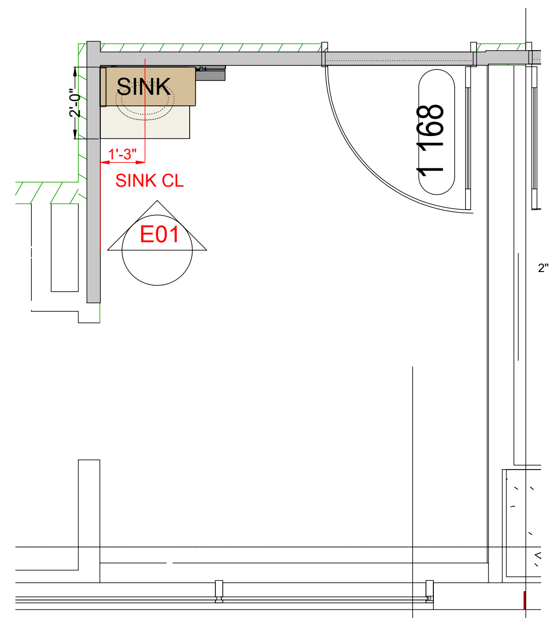
1 EXAM TYPICAL SINK LEFT PLAN VIEW SCALE: 3/8"=1" ROOMS INCLUDED: 1168 QTY 1 TOTAL
