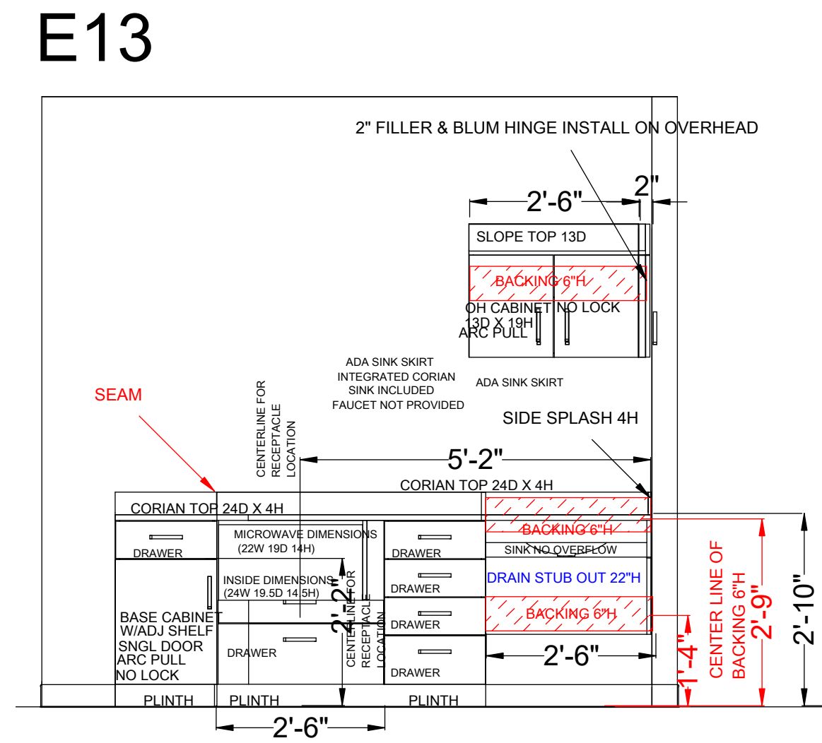
E13 NOURISH ELEVATION VIEW SCALE: 1/2"=1"
