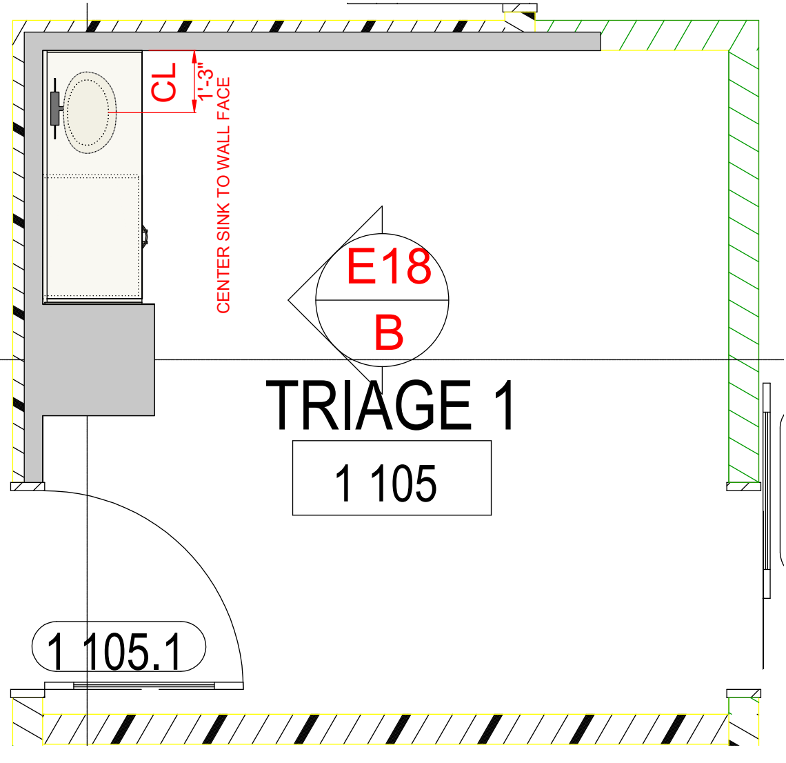
18 TRIAGE 1 PLAN VIEW SCALE: 3/8"=1"
