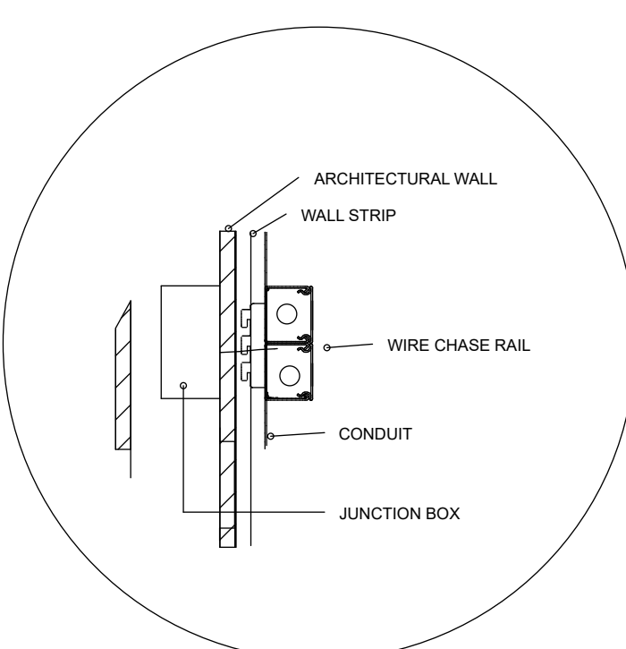
WIRE CHASE WALL ENTRY (WALL STRIP MOUNT) 1/4" = 1'-0"
