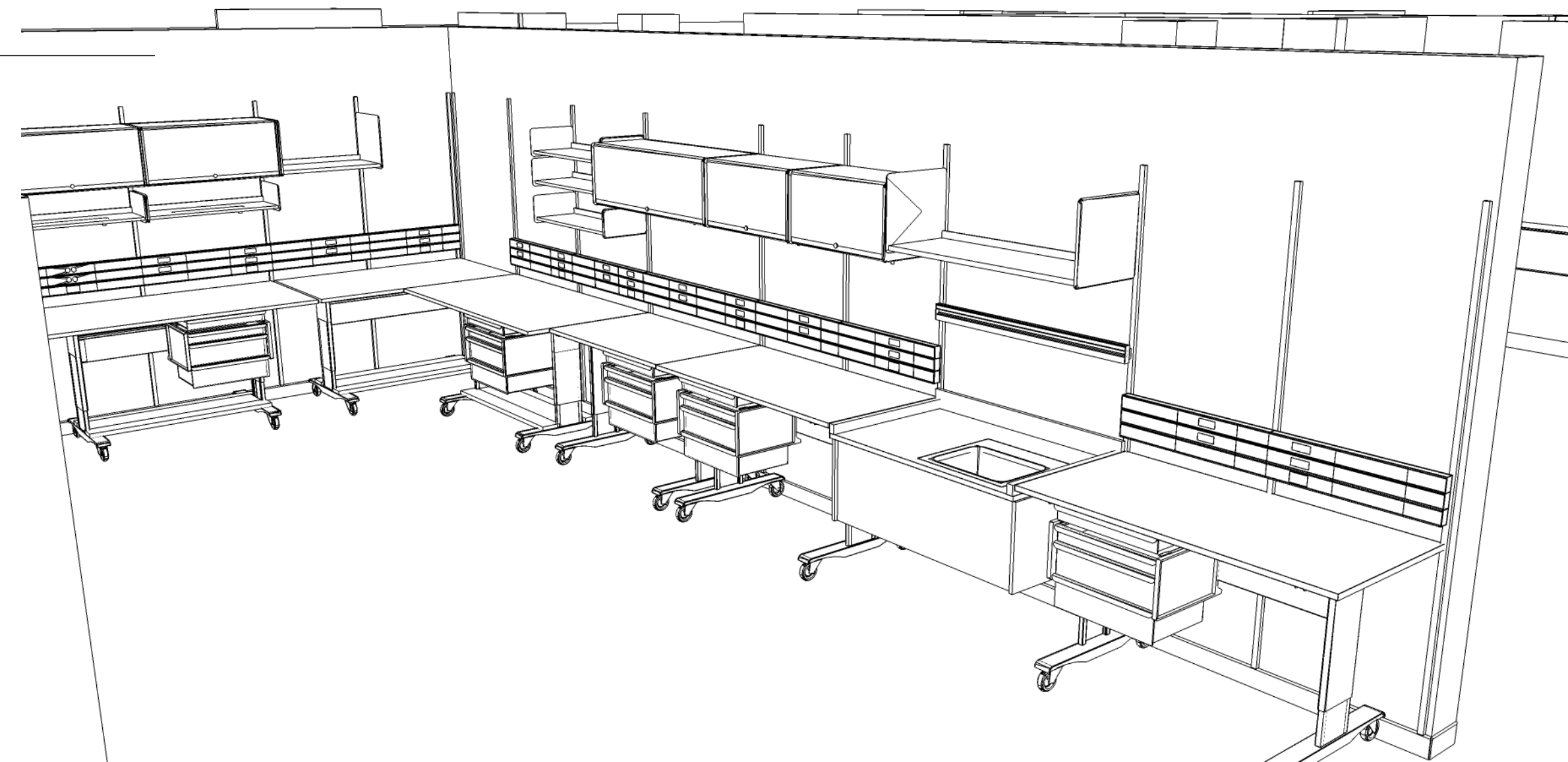
A LAB ISOMETRIC VIEW SCALE: NTS
