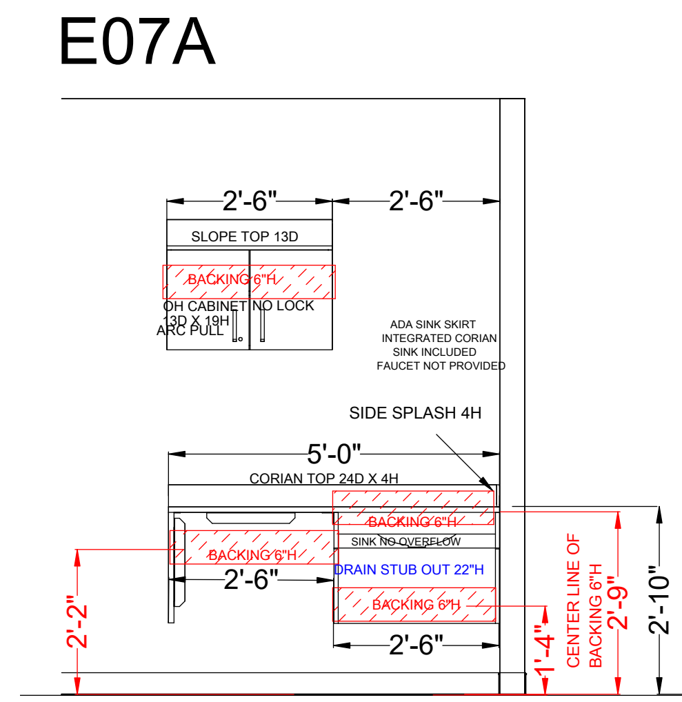
E7A RESUS 12 ELEVATION VIEW SCALE: 1/2"=1"
