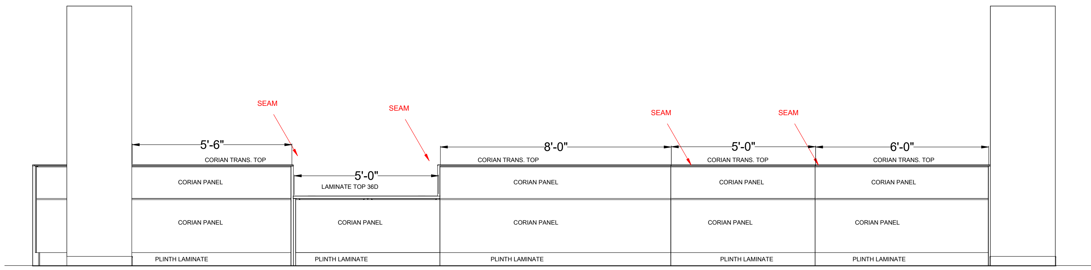
N4 NURSE STATION ELEVATION VIEW SCALE: 1/2"=1"
