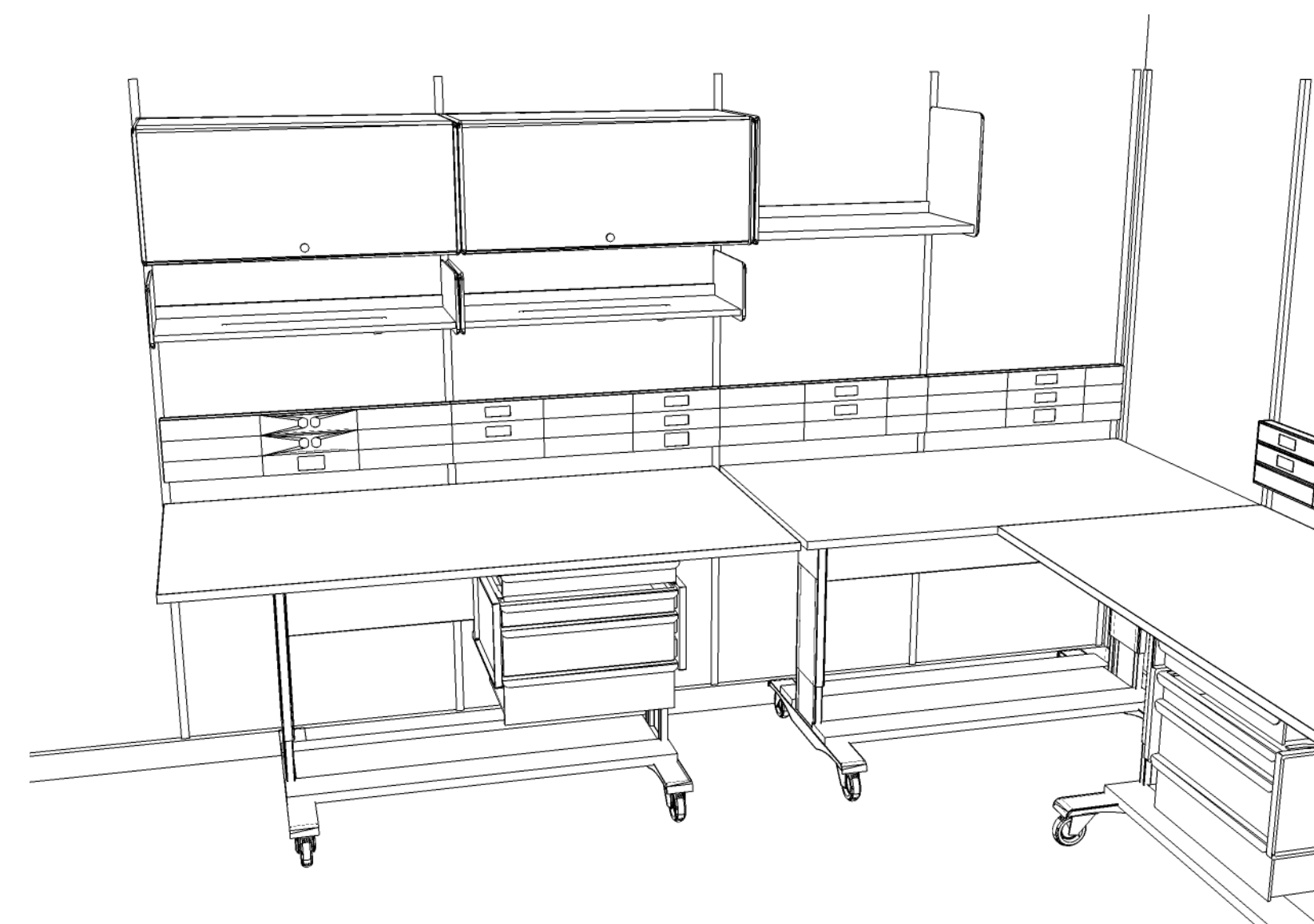
B LAB ISOMETRIC VIEW SCALE: NTS
