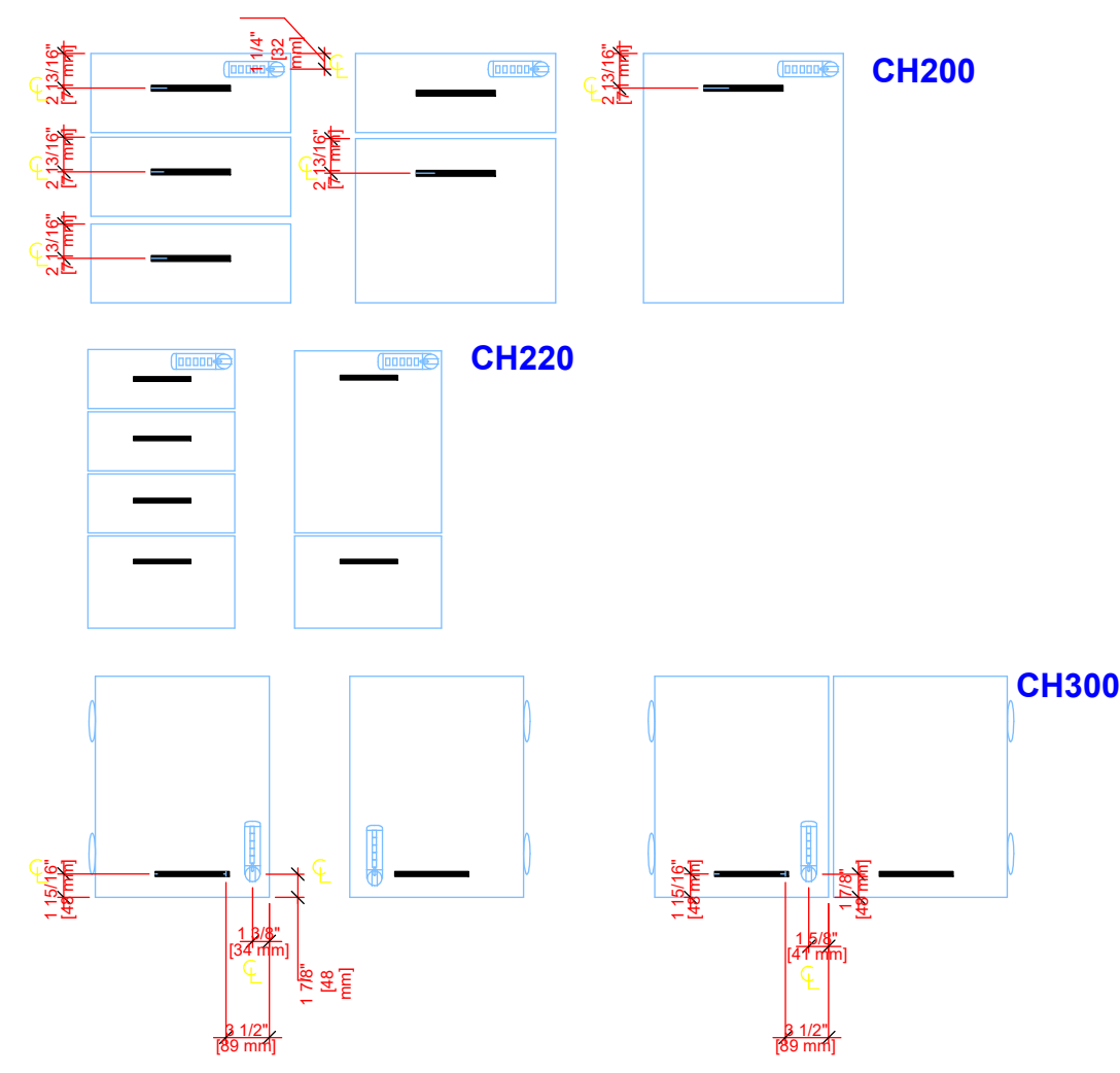
PULLLOCK LOCATIONS AND ORIENTATIONS 3/4\"/>
