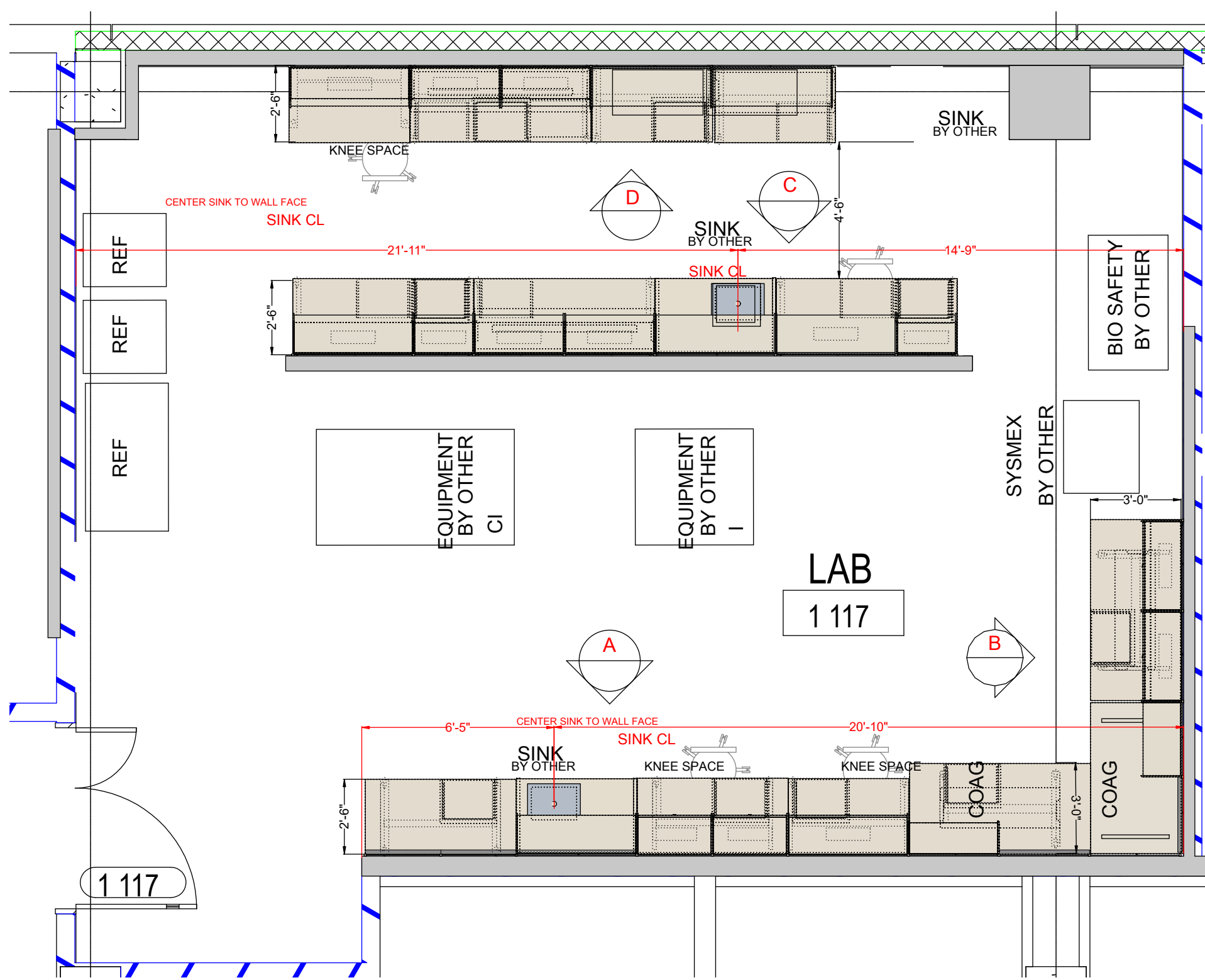
L LAB PLAN VIEW SCALE: 1/4"=1'
