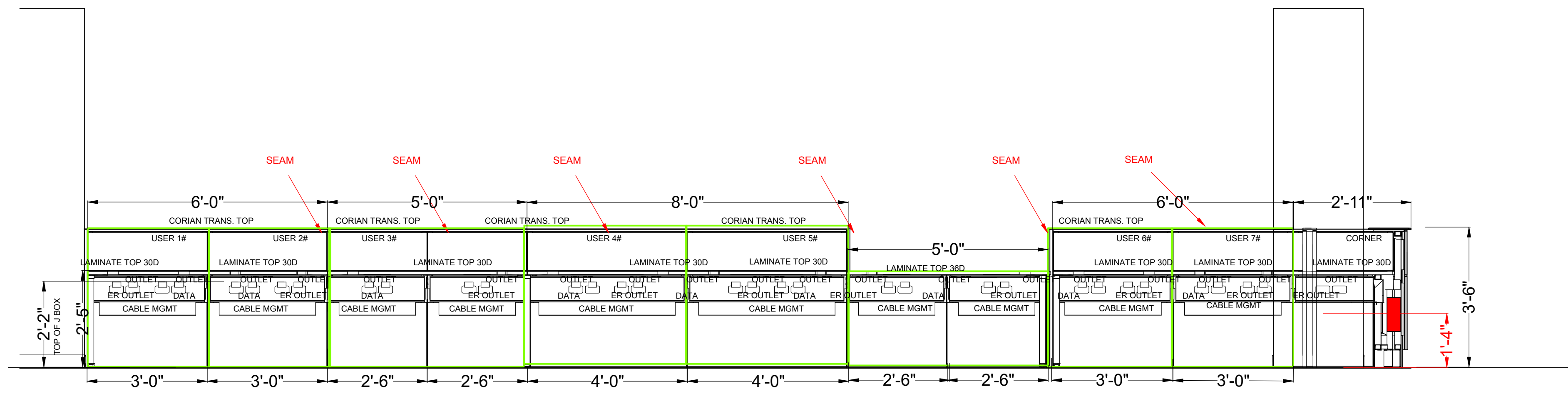
U4 NURSE STATION ELEVATION VIEW SCALE: 1/2"=1"
