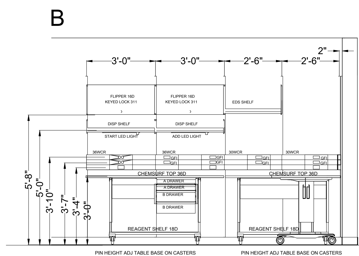
B LAB ELEVATION VIEW SCALE: 1/2"=1'
