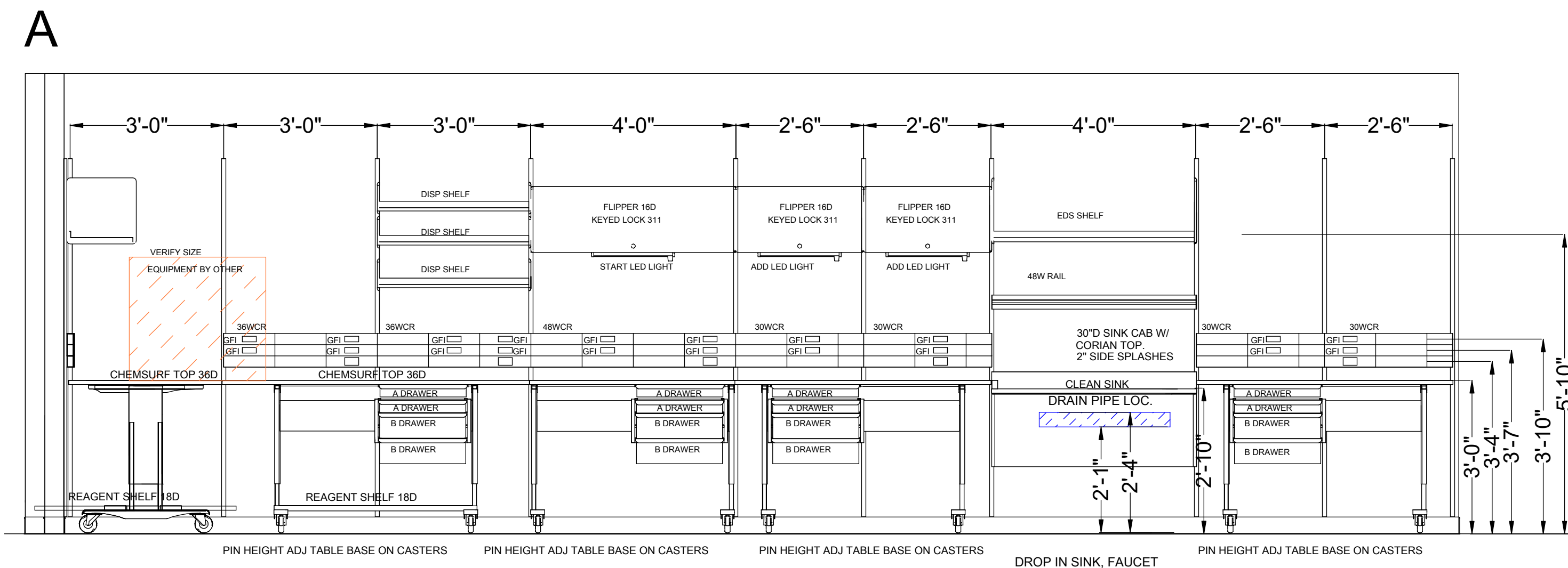
A LAB ELEVATION VIEW SCALE: 1/2"=1'
