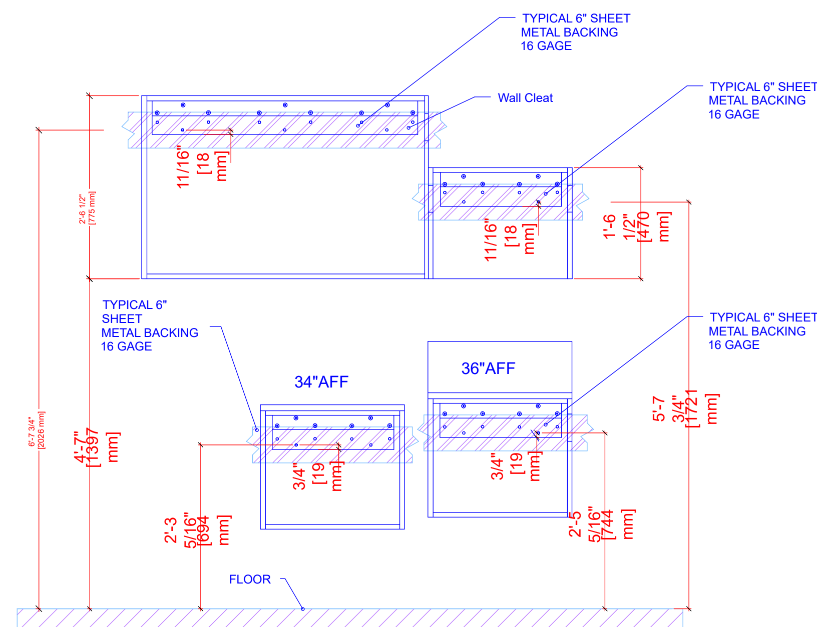
Backing Detail: Wall Mounted Cabinets 3/4\"/>
