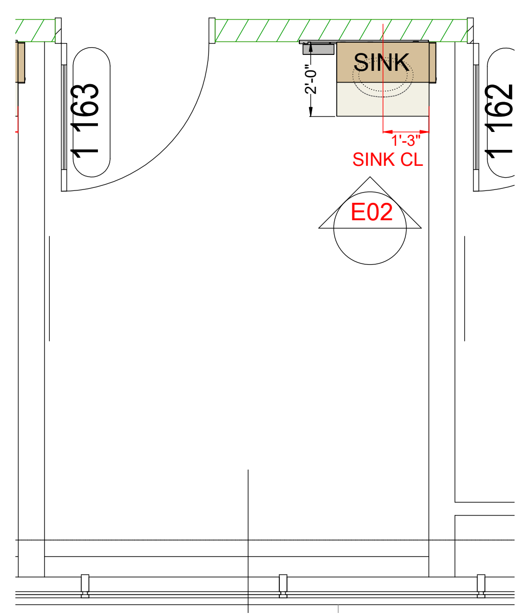
2 EXAM TYPICAL SINK RIGHT PLAN VIEW SCALE: 3/8"=1" ROOMS INCLUDED: QTY 19 TOTAL
