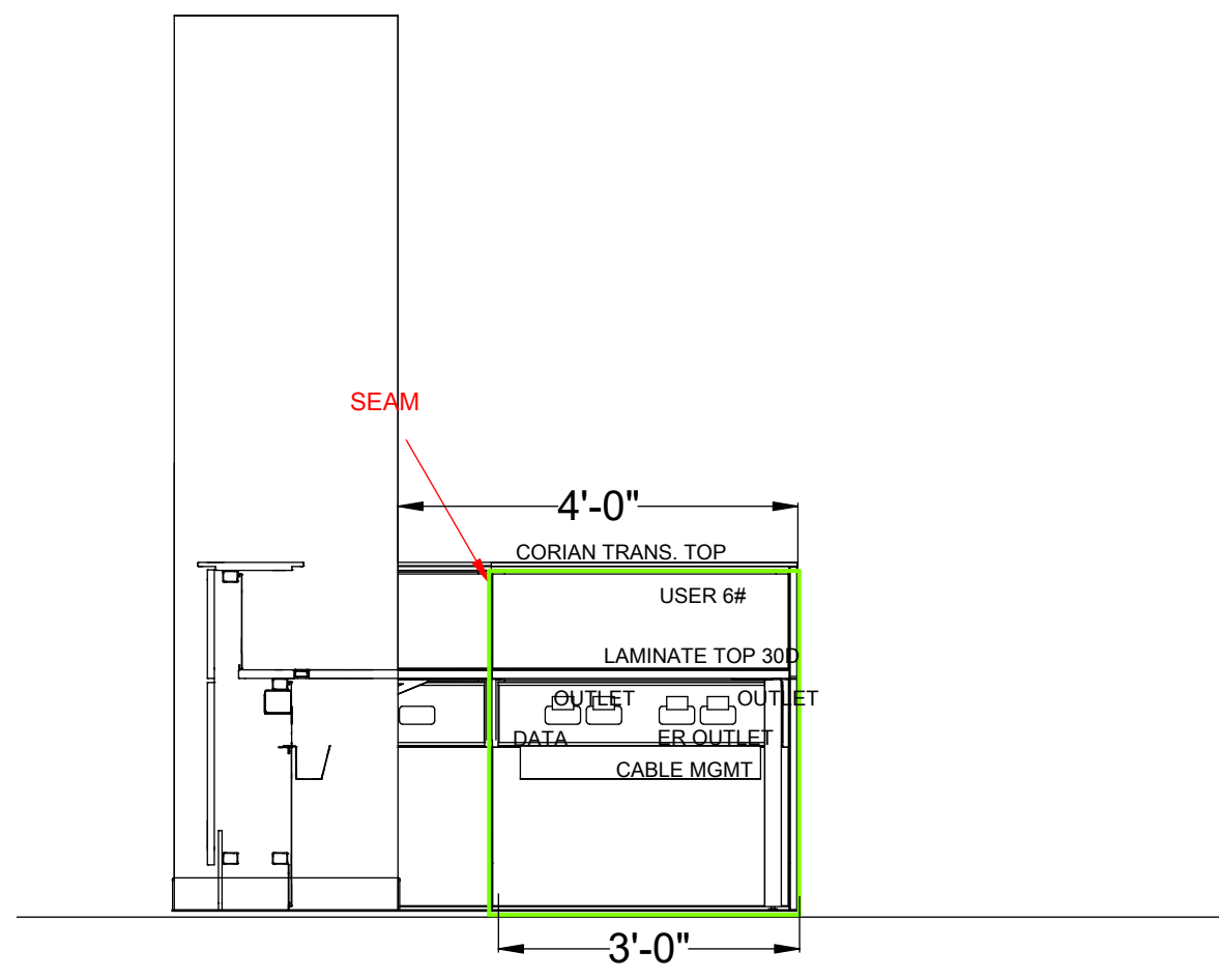
U4 NURSE STATION ELEVATION VIEW SCALE: 1/2"=1"
