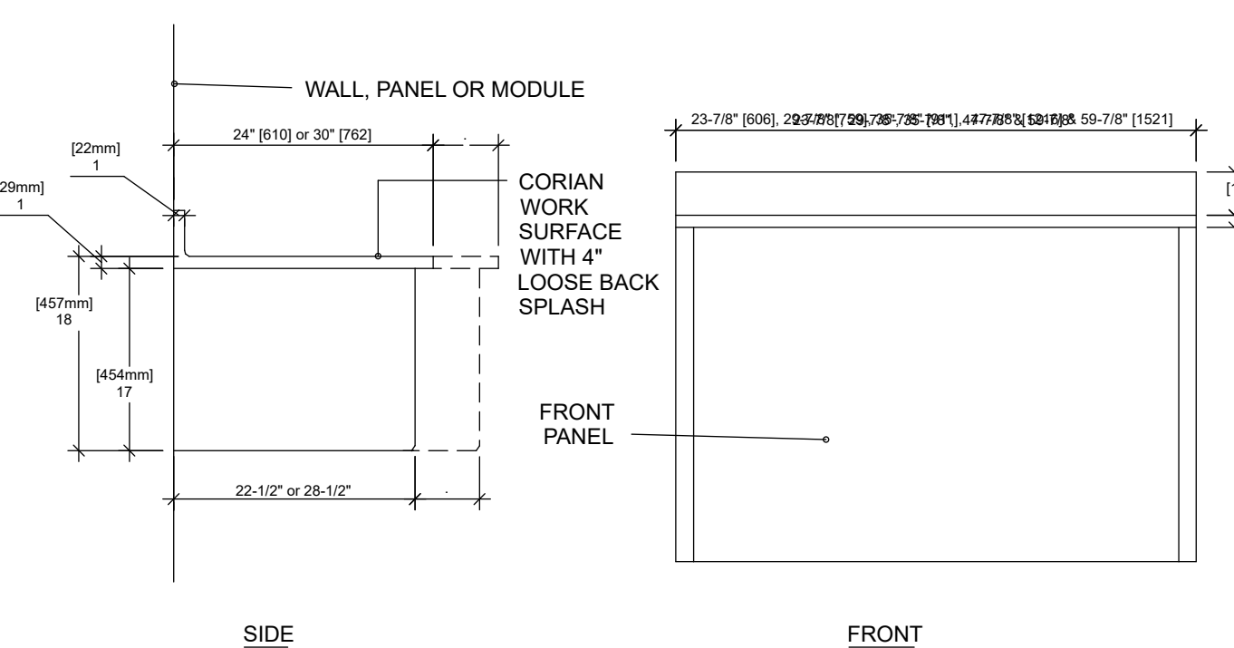
CO/STRUC SINK MODULE 3/4" = 1'-0"
