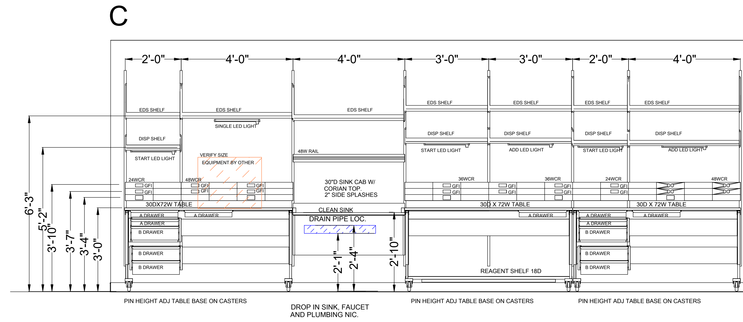
C LAB ELEVATION VIEW SCALE: 1/2"=1'
