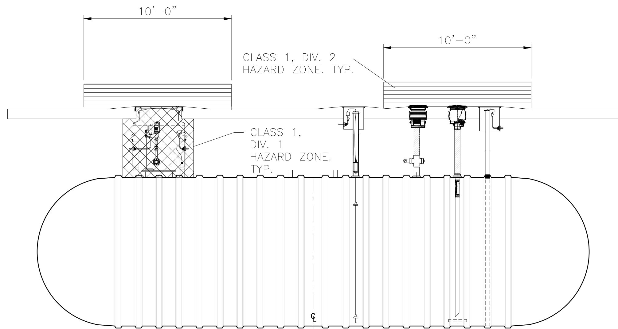
PROFILE
