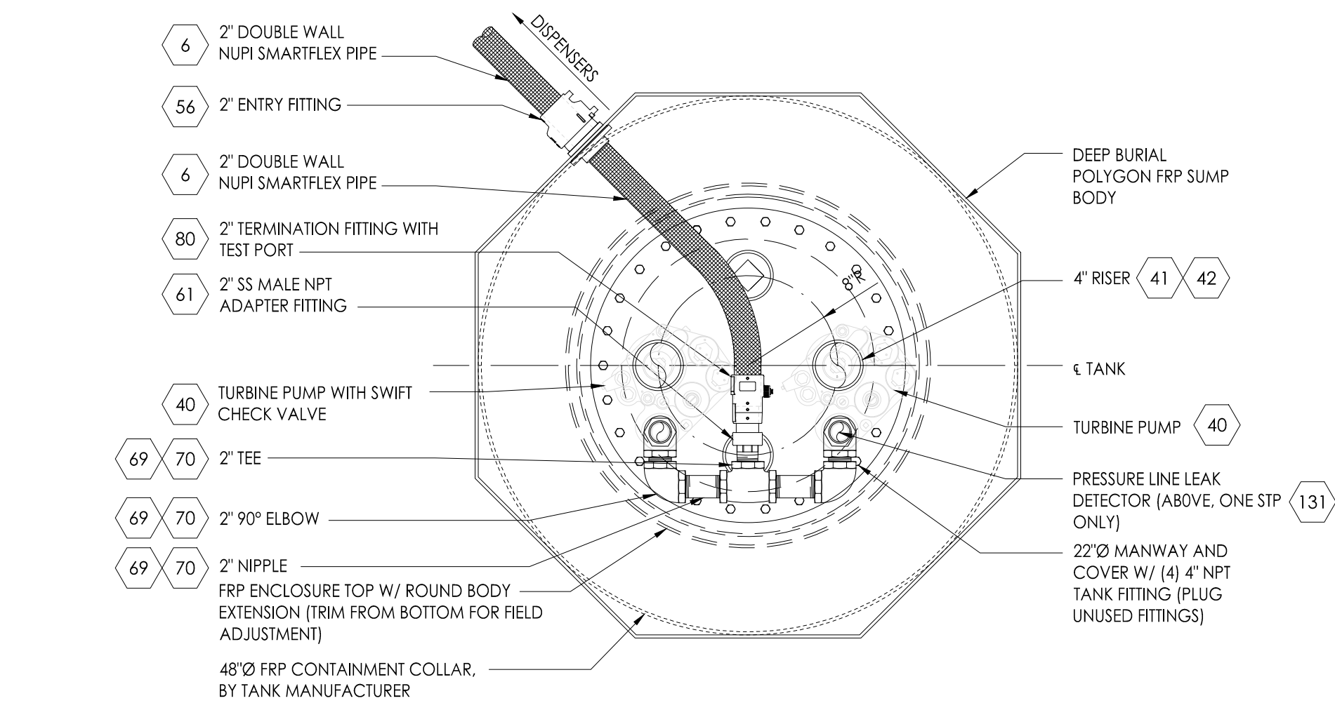
PLAN VIEW AT MANWAY
