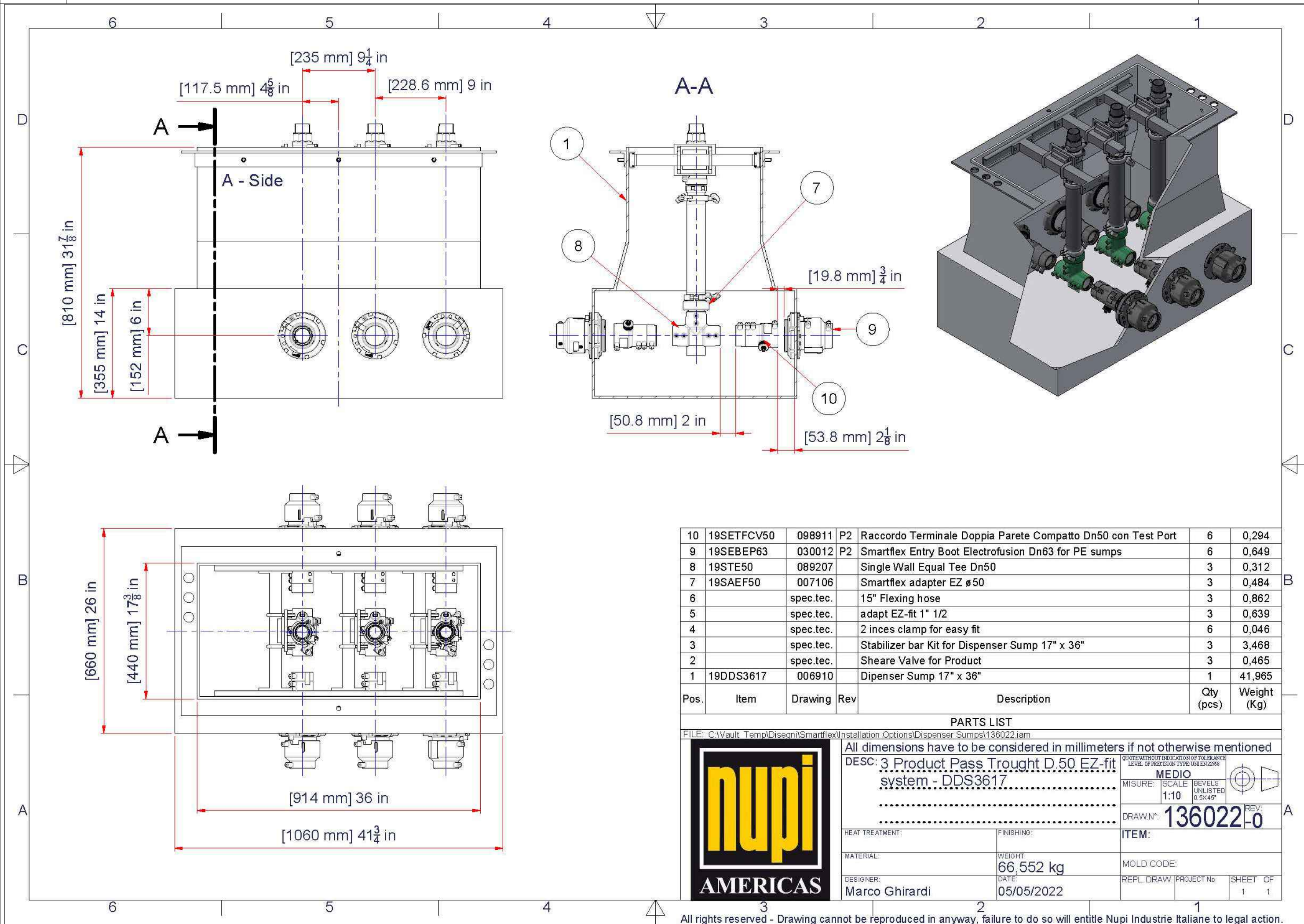
2 3+1 DISPENSER SUMP SECTION (THRU & THRU) SCALE: NTS
