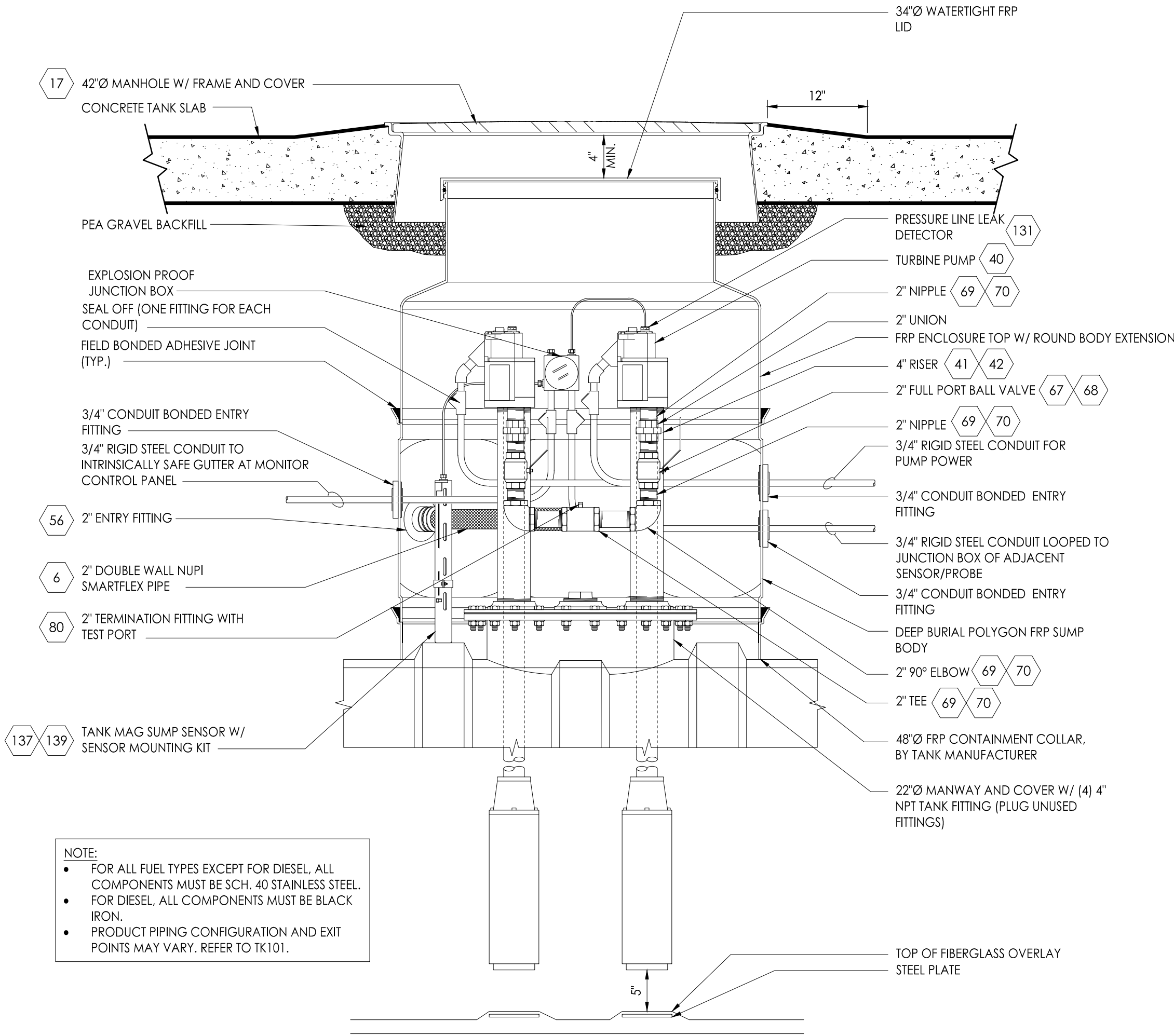
SECTION
