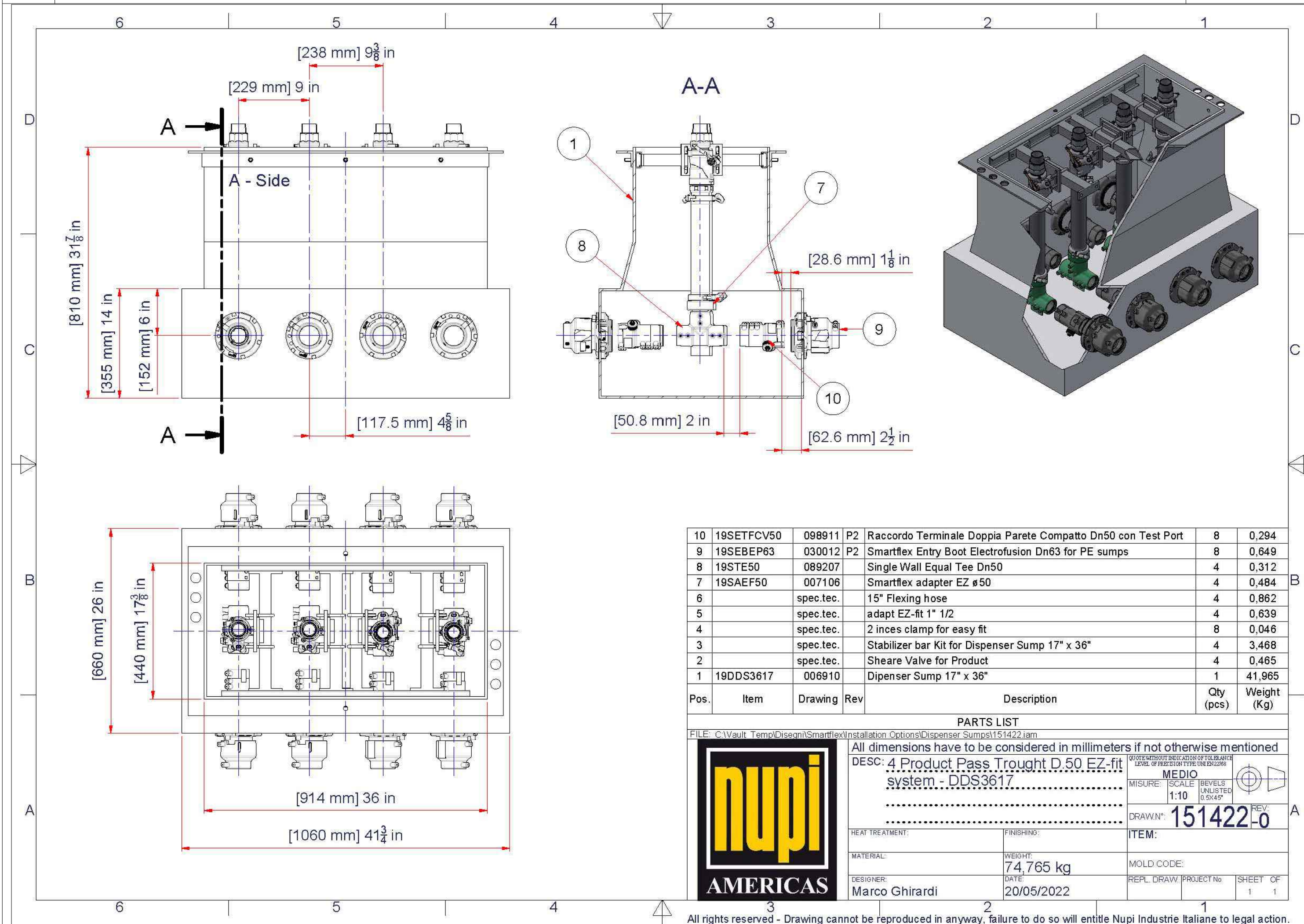
4 3+1+1 DISPENSER SUMP SECTION (THRU & THRU) SCALE: NTS
