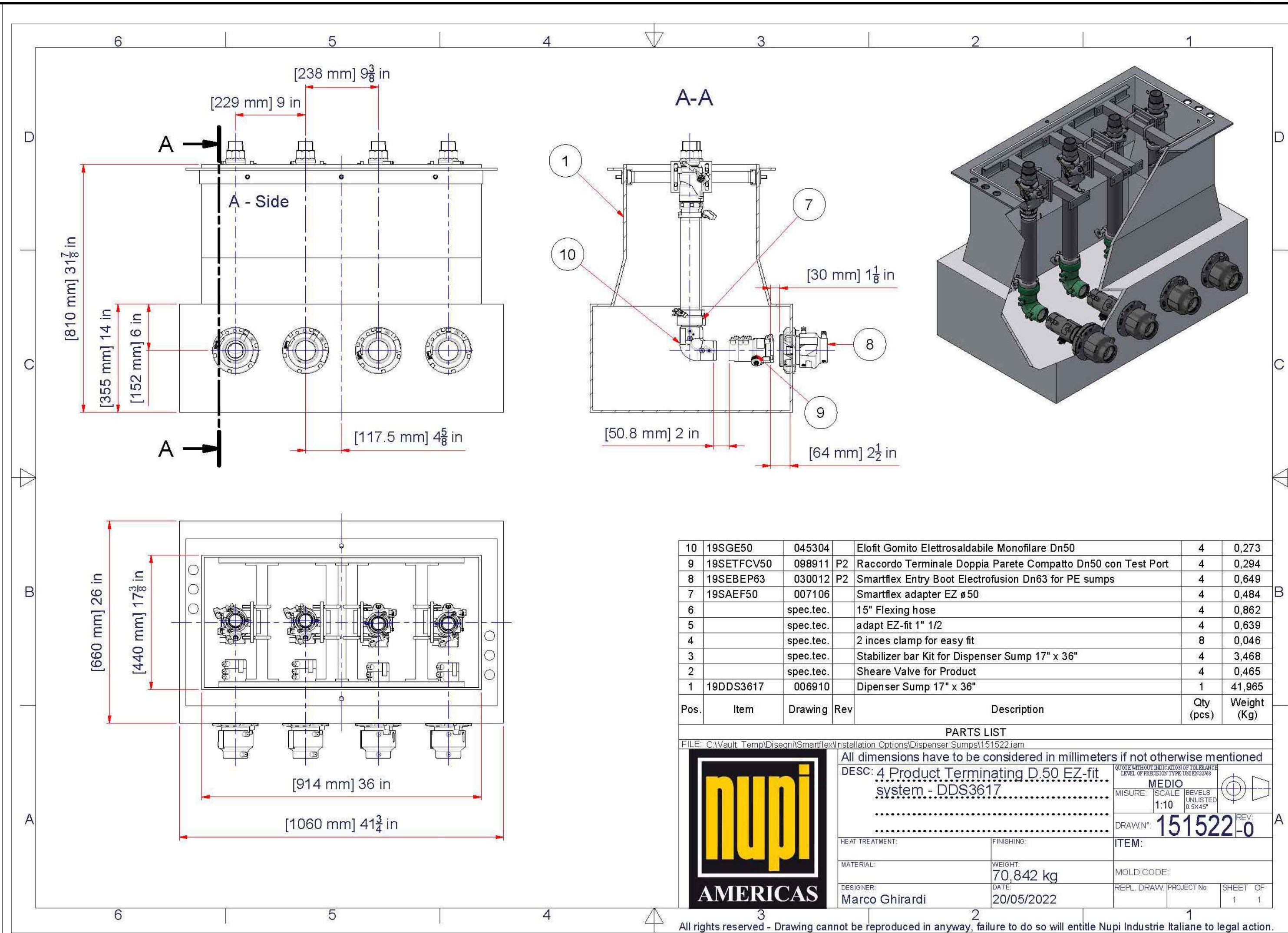
3 3+1+1 DISPENSER SUMP SECTION (TERMINATION) SCALE: NTS
