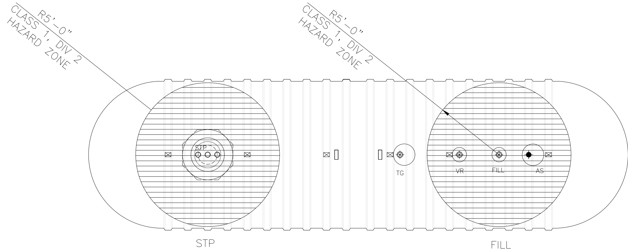
PLAN VIEW
