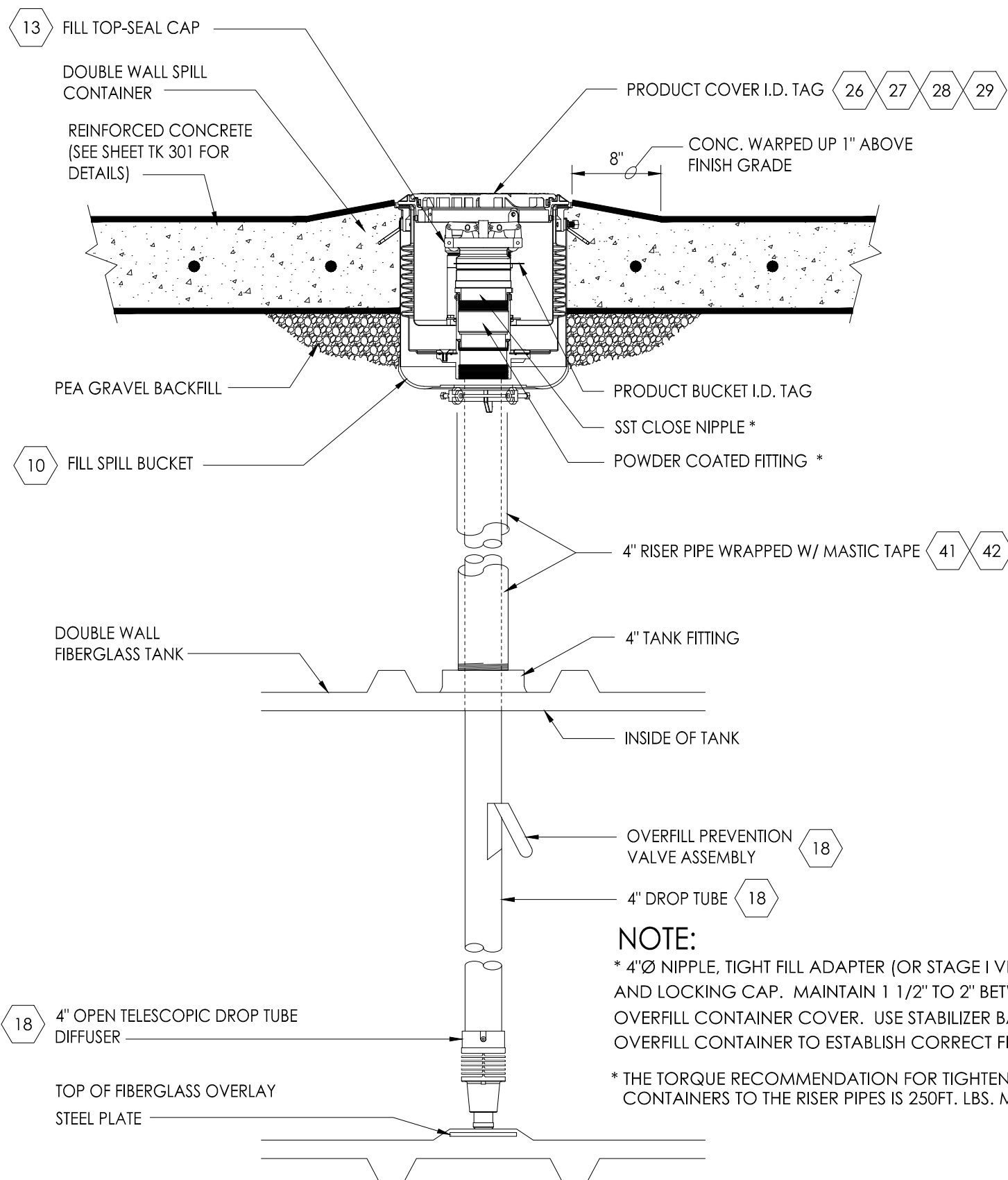
6 FILL RISER DETAIL
