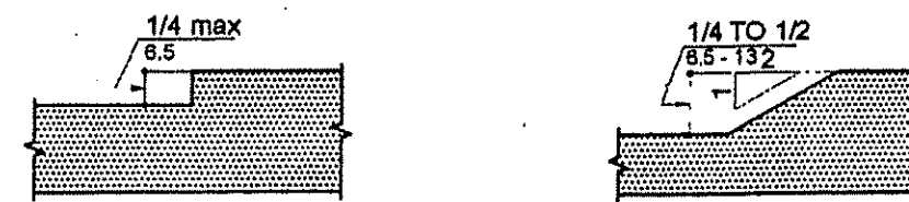
(c) Changes in Level
