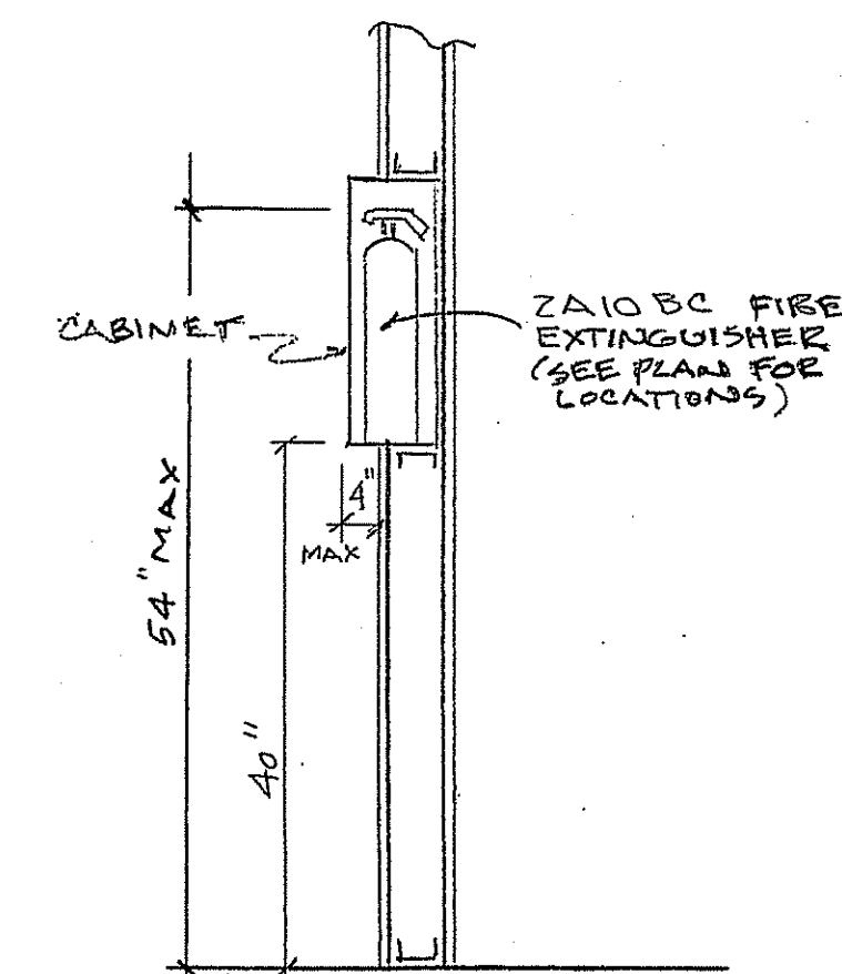
FIRE EXTINGUISHER (FE) CABINET DETAIL 3/4"
