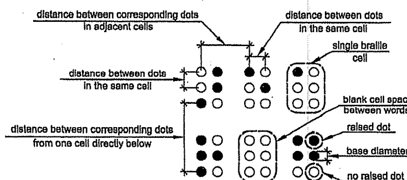
FIGURE 703.3.1 BRAILLE MEASUREMENT
