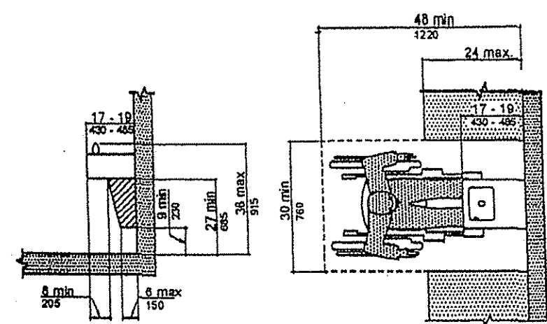
(a) Spout Height and Knee Clearance
