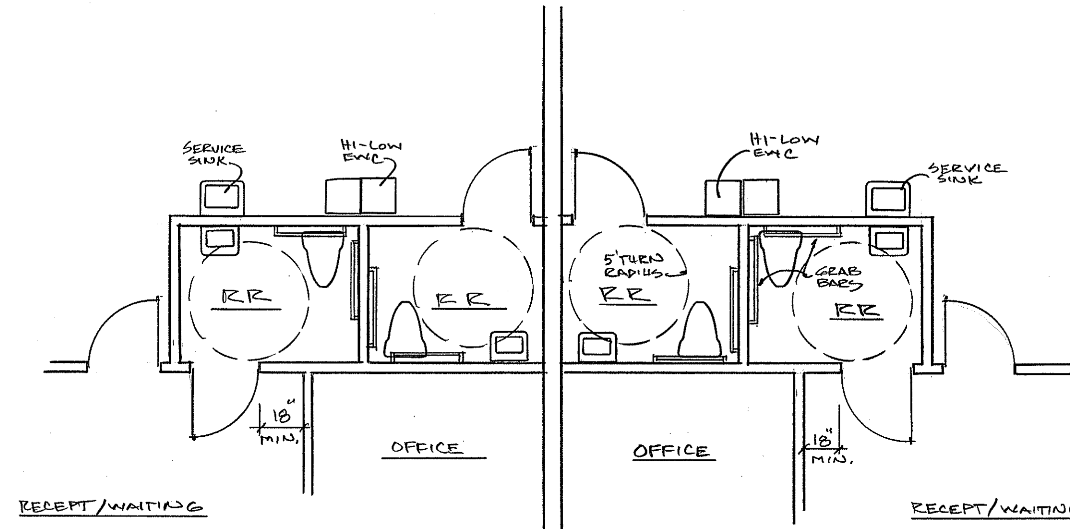
ENLARGED RESTROOM PLAN 1/4"
