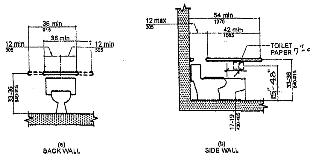
GRAB BARS AT WATER CLOSETS
