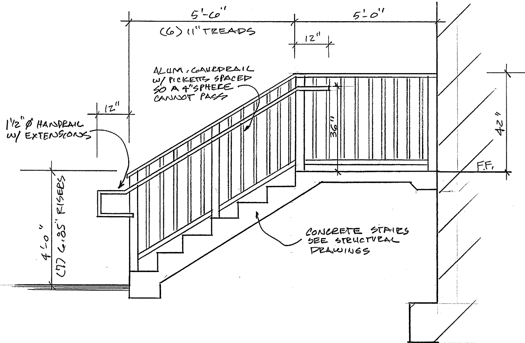
STAIR SECTION 1/2"
