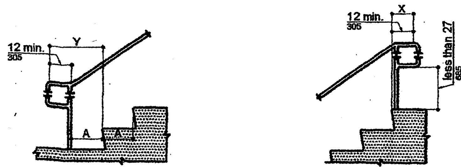
(c) Extension at Bottom of Run
