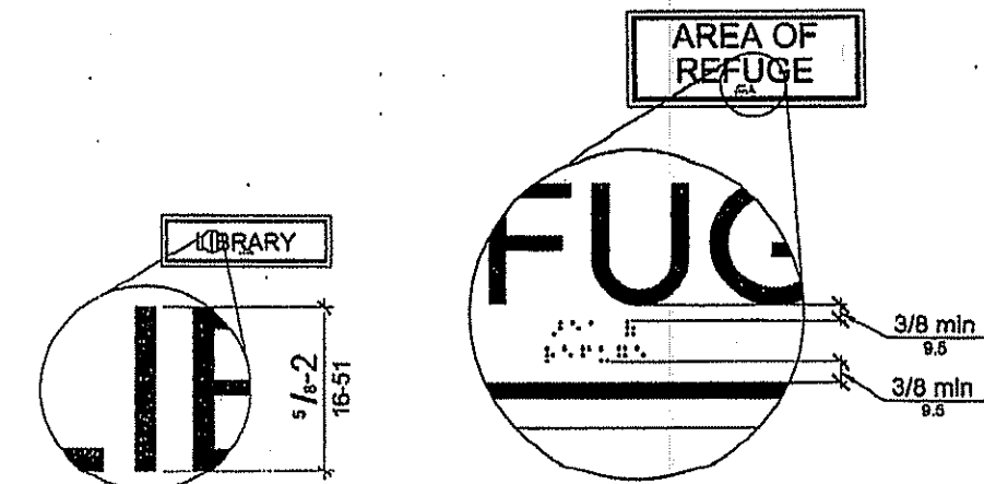
FIGURE 703.2.5 HEIGHT OF RAISED CHARACTERS
