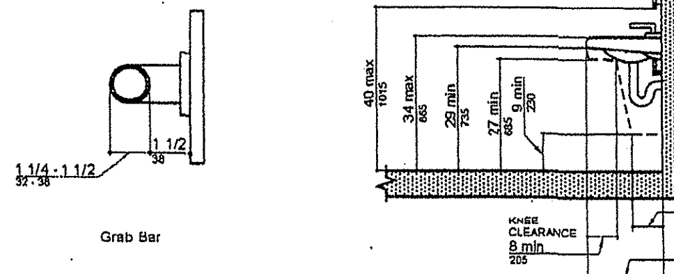
LAVATORY CLEARANCES NTS
