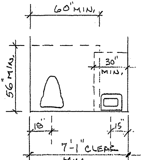
RESTROOM FIXTURE CLEARANCE DETAIL 1/4"
